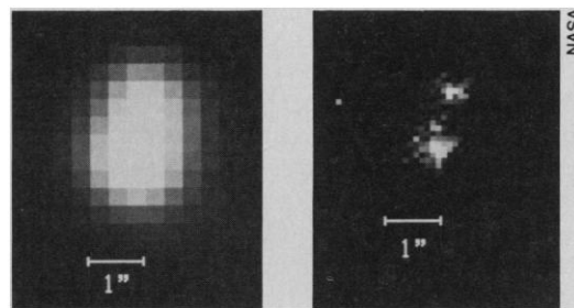
NGC 3532 viewed from the ground (left) and space.
