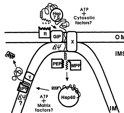
Fig. 1. Model for the import and sorting of cytochrome b 2 to the intermembrane space. Precursor cytochrome b 2 has a bipartite presequence whose NH 2 -terminal part (zigzag line) is positively charged and contains the information for the targeting into the matrix. The COOH-terminal part of the presequence (hatched box) corresponds to a bacterial-type targeting signal and directs the export to the intermembrane space (IMS).
