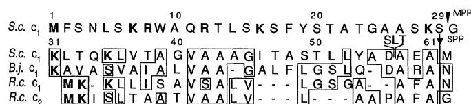
Fig. 2. Comparison of the presequence of yeast cytochrome c 1 (S.c. c 1 ) (49) with bacterial export signals. B.j. c 1 , cytochrome c 1 of Bradyrhizobium japonicum (64); R.c. c 1 , cytochrome c 1 of Rhodobacter capsulata ; R.c. c 2 , cytochrome c 2 of R. capsulata (63). The NH 2 -terminus of the precursor of B.j. c 1 has not been precisely determined (64). Amino acids are shown by the one-letter code (92); positively charged residues shown in bold print. Shaded boxes indicate identical amino acid residues. Dashes represent gaps introduced to maximize sequence alignment. Amino acid residues in the precursor of S.c. c 1 are numbered starting with the first amino acid of the presequence. MPP, putative cleavage site of the mitochondrial processing peptidase (2, 46). SPP, cleavage sites of the mitochondrial and bacterial signal peptidases.
