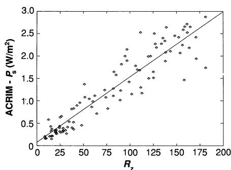
Fig. 4. Regression of ACRIM irradiance residuals, S - P_s , against R_z . Monthly averaged data are used for the period from March 1980 to December 1988. \text{ACRIM} - P_s = 0.078 + 0.0146 R_z ; uncertainty (SE) in slope = 0.0006.
