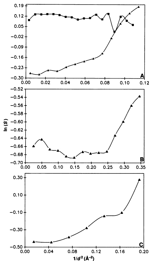
Fig. 2. Relative Wilson plot ( \Delta ) comparing space-grown and Earth-grown crystals of (A) \gamma -IFN D 1 , (B) porcine elastase, and (C) isocitrate lyase. In addition, a relative Wilson plot ( \blacksquare ) comparing two Earth-grown crystals of \gamma -IFN D 1 is shown in (A). S = \Sigma F_a^2 / \Sigma F_b^2 .
