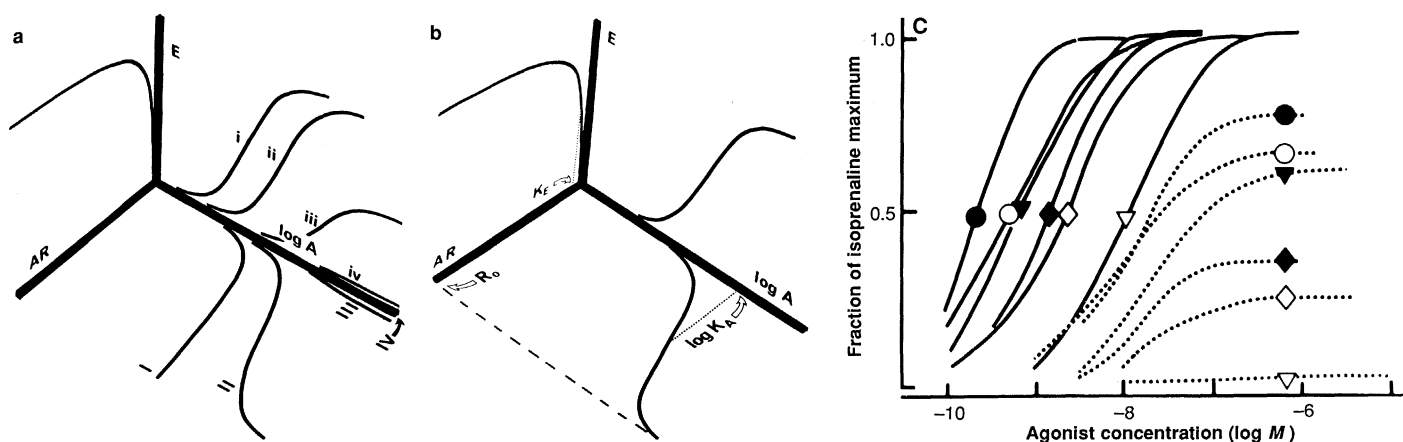
Fig. 12. (a) Three-dimensional display of the operational model of agonism (28). E , pharmacological effect; \log A , logarithmic concentration of agonist A ; \log K_A , log equilibrium agonist dissociation constant; R_0 , operational receptor concentration; AR , concentration of receptors occupied by A ; K_E , concentration of AR required for half-maximal tissue response. The three planes of the figure represent pharmacological effect (right panel), binding or affinity (base panel), and efficacy or transduction (left panel). (b) Predictions of the influence of changes in R_0 concentration on pharmacological effect by the use of the operational model of agonism. Curves I to IV show R_0
