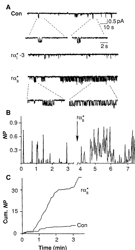
Fig. 1. Activation of skeletal muscle T-tubule \text{Ca}^{2+} channels by the recombinant short 379 amino acid \alpha_s fusion polypeptide [ \text{r}(+9)\alpha_s -S1] but not by the recombinant \alpha_i -3 fusion polypeptide [ \text{r}(+9)\alpha_i -3]. \text{Ca}^{2+} channels from skeletal muscle T tubules were incorporated into planar lipid bilayers and single-channel trans to cis currents were measured at a holding potential of 0 mV using \text{Ba}^{2+} as the charge carrier (9). Baseline currents were recorded for 5 to 10 min. Preparations of \text{r}(+9)\alpha_s -S1 and \text{r}(+9)\alpha_i -3, activated by treatment with GTP \gamma S, purified partially by DEAE-Sephacel chromatography (7), and concentrated by ultrafiltration (12), or control (Con) solutions, were added as 10- to 20- \mu l aliquots to the 0.2-ml cis chamber and recording was continued for an additional 5 to 10 min or until the bilayer broke down. (A) Single-channel \text{Ca}^{2+} currents displayed at two time resolutions were recorded during a control period before addition of recombinant \alpha subunits, after the addition of 4 nM partially purified GTP \gamma S-activated recombinant \alpha_i -3 protein prepared by the plasmid-phase method [ \text{r}(+9)\alpha_i -3], and after addition of 2.4 nM partially purified GTP \gamma S-activated \text{r}(+9)\alpha_s -S1 protein (28 pM G_s equivalents of \text{cyc}^- reconstituting activity). (B) Average currents from incorporated \text{Ca}^{2+} channels before and after addition of 4 nM GTP \gamma S-activated \text{r}(+9)\alpha_s -S1 protein (equivalent G_s activity = 34 pM) prepared by the two-plasmid method. The probability of an opening event, P , produced by any one of N incorporated channels was calculated from records such as those shown in (A) to give NP values. If one assumes the unitary amplitude to be constant, which is reasonable because the 10-pS conductance accounts for about 90% of all openings (1), NP represents the current. NP was integrated every 0.5 s to produce the experimental diary shown. (C) Cumulative NP values computed from the experiment in (B). The effect of \text{r}(+9)\alpha_s -S1 shown is representative of more than 20 other such experiments.
