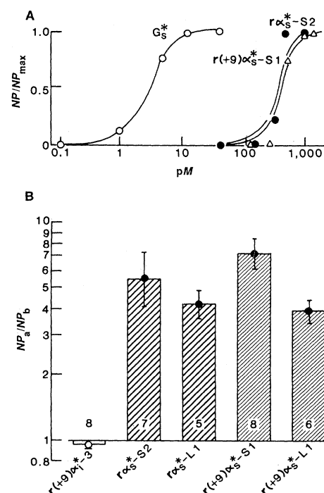
Fig. 2. Stimulation of \text{Ca}^{2+} channel activity by individual recombinant \alpha_s splice variants. (A) Concentration-effect curves for stimulation of single-channel \text{Ca}^{2+} currents by GTP \gamma S-activated forms of G_s and two recombinant splice variants. hRBC G_s^* ; GTP \gamma S-activated native G_s from human erythrocytes; \alpha_s -S2, purified; GTP \gamma S-activated recombinant 380-amino acid \alpha_s prepared by the two-plasmid method; \text{r}(+9)\alpha_s -S1, partially purified GTP \gamma S-activated recombinant 379-amino acid \alpha_s with 9-amino acid amino-terminal extension, prepared by the plasmid-phase method. Each point is the average of two measurements, and the points were normalized to the maximum value. (B) Relative stimulations of incorporated \text{Ca}^{2+} channels by recombinant splice variants expressed as ratios of NP after addition of the recombinant GTP \gamma S-activated polypeptides to NP before their addition ( NP after/ NP before). Values are geometric means \pm SEM of the number of experiments shown. The concentrations of recombinant subunits used varied between 0.6 and 4 nM of recombinant polypeptides ( \alpha_s -S2, \alpha_s -L1) or 2 to 10 pM equivalents of human erythrocyte G_s activity [ \text{r}(+9)\alpha_s -S1 and \text{r}(+9)\alpha_s -L1]. GTP \gamma S-activated \text{r}(+9)\alpha_i -3 [ \text{r}(+9)\alpha_i -3] at 0.5 to 4 nM, added in some experiments before addition of the recombinant \alpha_s subunits, was always without effect.
