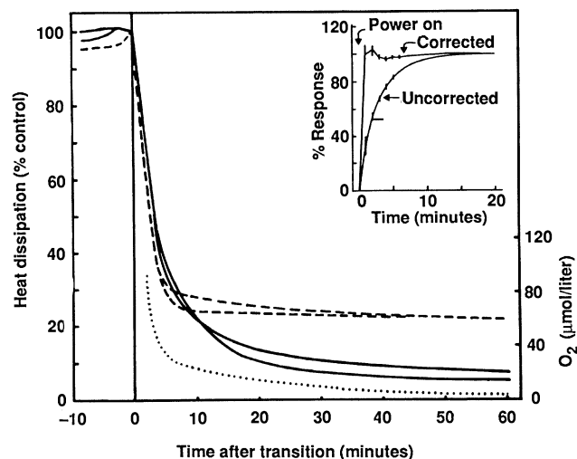
Fig. 3. High resolution of the time course of heat dissipation during p\text{H} -induced metabolic transitions in Artemia embryos. Superimposed traces from two experiments are presented for each of the following conditions: aerobic acidosis (---) and anaerobic dormancy (—). Heat dissipation is calculated as percent of the aerobic control prior to each transition. Time course for washout of oxygen from the perfusion system after switching to anoxic medium is depicted by the dotted line. The inset shows the accuracy of time resolution for the calorimetry signal achieved by correcting for instrumental lag (29). The internal calibration heater was activated at time 0 ("Power on"). Vertical bars represent \pm 1 SD ( n = 10 ).
