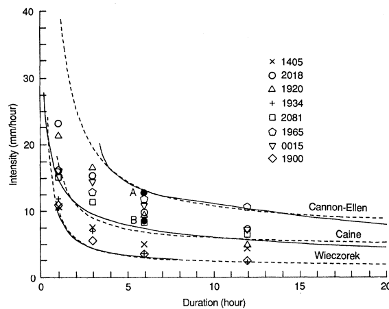
Fig. 2. Rainfall intensity and duration thresholds for initiation of debris flows on susceptible slopes. Published empirical curves are shown by solid lines; curves resulting from numerical fitting by using Eq. 5 are shown as dashed lines. The Cannon-Ellen threshold is for abundant debris flows from natural slopes in areas of the San Francisco Bay region having average annual precipitation greater than 660 mm (14). The Caine threshold is for individual debris flows on natural slopes based on worldwide data (11). The Wiczorek threshold is for individual debris flows near La Honda, California (13), site of ALERT rain gage 1405 in Fig. 1. Also plotted are points indicating the maximum rainfall intensities for intervals of 1, 3, 6, and 12 hours recorded at various ALERT rain gages in and near landslide areas during the 12 to 21 February 1986 storms; numbers beside the symbols denote the various ALERT gages, situated as shown in Fig. 1. Points A and B are the 6-hour rainfall forecasts noted in the warning issued at noon on 14 February; point A was the maximum forecast for the region, and point B was the specific forecast for the Lexington Burn area.
