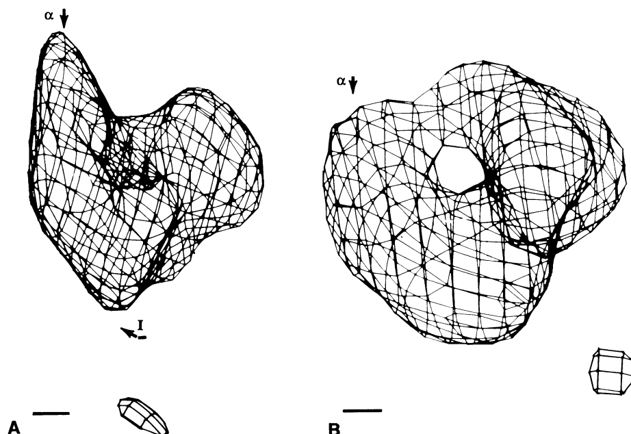
Fig. 5. The model obtained from three-dimensional image reconstruction at 55 Å resolution (part of the data used for Fig. 3A). (A) The view is from approximately the same direction as in Fig. 3B. Part of the second particle is shown and marked by I. (B) A view into the tunnel from the cleft. Bar length, 20 Å.
