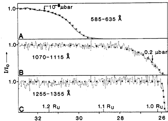
Fig. 1. Light curves measured in the occultation observations. The abscissa is distance measured from the center of the planet (× 10 3 km) referred to a common geopotential at the equator. The model fits (X) were computed from the altitude profiles in Fig. 2. (A) Solar occultation, H 2 continuum; (B) γ Pegasi occultation, H 2 band absorption; (C) γ Pegasi occultation, CH 4 absorption.
