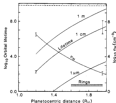
Fig. 6. Hydrogen number density and orbital lifetimes (in years) of particles of various sizes as a function of distance from the center of Uranus. The uncertainties in hydrogen density and orbital lifetimes corresponding to the \pm 100 K uncertainty in exospheric temperature are indicated by the error bars. The dashed line represents the age of the solar system.
