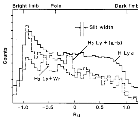
Fig. 4. Brightness profiles across the sunlit hemisphere of Uranus on 24 January 1986 U.T. H Lyman \alpha , 1216 Å; H 2 Ly + Wr, 902 to 1115 Å; H 2 Ly + (a-b), 1273 to 1514 Å.
