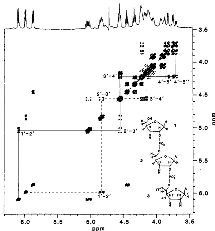
Fig. 5. Double-quantum filtered absorption mode (270 MHz) 2-D COSY spectrum of the ribose region of the trinucleotide \text{A2}'\text{-P-5}'\text{A2}'\text{-P-5}'\text{A} , with the conventional ^1\text{H} spectrum shown along the top axis. The solid lines indicate connectivity within the sugar ring of nucleotide 1, the broken line is for the sugar ring of 2. The total measuring time for this spectrum was 3 hours. A, adenine.
