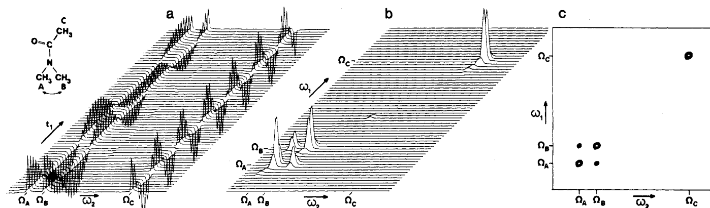
Fig. 3. The generation of a 2-D exchange spectrum of N,N -dimethylacetamide, from data obtained with the pulse sequence of Fig. 2a (the mixing time was 500 msec). After Fourier transformation with respect to t_2 , a set of spectra modulated in amplitude as a function of t_1 is obtained (a). A Fourier transformation, with respect to t_1 , of the columns of the data matrix corresponding to this set of spectra yields resonances at the modulation
