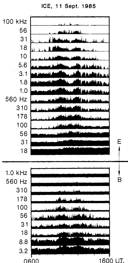
Fig. 2. Details of the E- and B-wave measurements within 375,000 km of closest approach. Each panel has a plot of the peak amplitude measured in a 128-second interval. For all 16 E-field channels and the top eight B-field channels the vertical scale corresponds to a variation of nine orders of magnitude in wave energy; the two lowest frequency B-field channels (which show saturation here) have somewhat smaller dynamic ranges. Since launch in August 1978, the ICE plasma wave instrument never detected stronger signals than those shown here.
