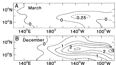
Fig. 2. March and December SST anomalies during the model El Niño event in year 31. (Note that the contour interval for March is 0.25°C and that for December is 0.5°C.)
