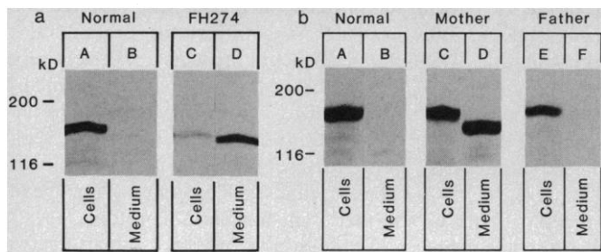
Fig. 9. Recovery in the culture medium of newly synthesized LDL receptor from fibroblasts of FH 274 (a) and his mother and father (b). Fibroblasts from the indicated subject were induced for LDL receptor synthesis as described in Fig. 8. Cells were labeled
