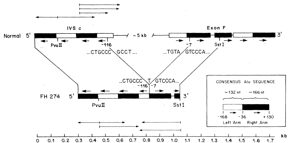
Fig. 4. Strategy for sequencing and orientation of the relevant Alu repetitive sequences in the normal LDL receptor gene and the corresponding region from the deletion-bearing gene from FH 274. The upper and lower parts of the figure show the relevant regions of the normal and FH 274 genes used for DNA sequencing. These sequences (corresponding to the regions delimited by the solid bars in Fig. 3) were determined from the following clones: IVSc from \lambda 33-1 (10), exon F from the previously reported sequence of pLDLR-2 (9), and the FH 274 deletion joint from \lambda FH 274-10. DNA sequencing was performed by the dideoxy-chain termination method (24). The direction and extent of sequence established in a given experiment are indicated by the long arrows above or below the relevant DNA segments. Those sequences not coinciding with a restriction endonuclease site were determined with synthetic oligonucleotides as primers on M13 subclones (25). The boxed area shows a consensus Alu sequence with the left and right tandem repeats (open and closed, respectively). The nucleotide numbering scheme of the consensus Alu is the same as that described (11); position +1 refers to the C of the Alu I endonuclease recognition site, AGCT. Alu sequences in the normal and FH 274 genes are illustrated according to the same numbering scheme. Orientations of the left and right tandem Alu repeats are indicated by the short arrows. Segments of the normal and FH 274 genes that correspond to each other are connected by the diagonal lines. The exact DNA sequences around nucleotide positions -116 and -7 in the Alu repeats of IVSc and exon F, respectively, and of the deletion joint in FH 274 are shown.
