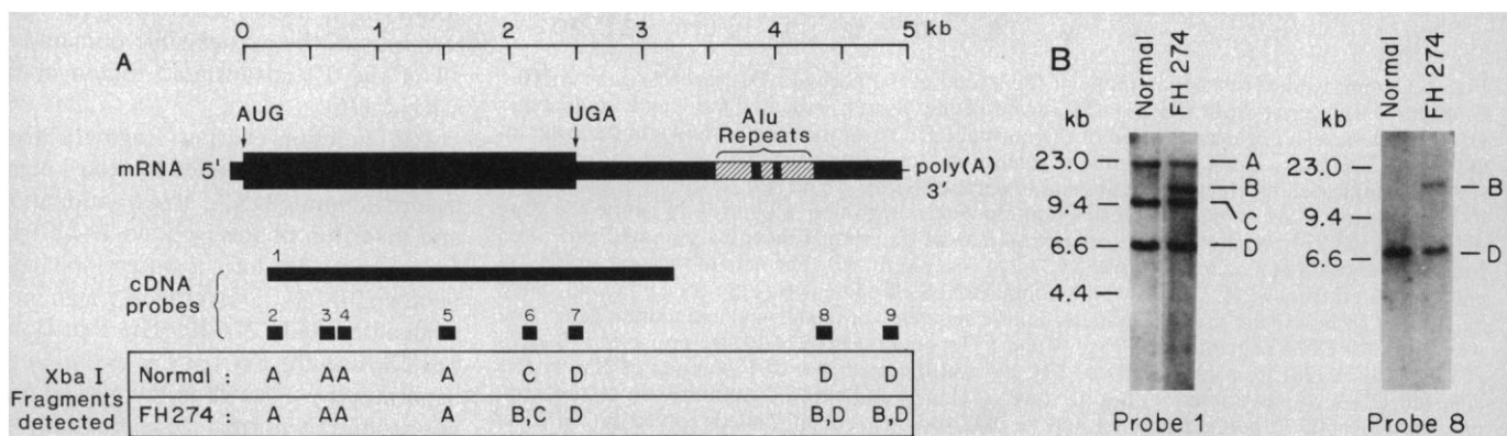
Fig. 1. Analysis of Xba I restriction digests of genomic DNA from FH 274 with probes from different regions of the LDL receptor cDNA. (A) A diagram of the mRNA for the human LDL receptor (9) is shown with AUG and UGA (A, adenine; U, uracil; G, guanine) indicating the beginning and end of the translated region. The hatched areas in the 3' untranslated region represent Alu repetitive sequences. The sizes and locations of 32 P-labeled cDNA probes used to map the LDL receptor gene are shown by the closed bars and are numbered 1 to 9. Probe 1 (double-stranded DNA) was a mixture of a 2.1-kb Eco RI-Sma I fragment and three different 0.9-kb Bam HI-Xho I fragments from p101 (9), which together spanned most of the translated region; the fragments were purified by polyacrylamide gel electrophoresis and electroelution (20) and then labeled with 32 P by random hexanucleotide priming (21). Probes 2 to 9 were prepared from M13 subclones of pLDLR-2 (9) as single-stranded, uniformly 32 P-labeled DNA, ~100 nucleotides (nt) in length, by the method of Church and Gilbert (22). All probes had a specific radioactivity of at least 5 × 10 8 cpm/μg. (B) Genomic DNA (5 μg) was isolated from cultured fibroblasts as indicated (20), digested with Xba I (New England Biolabs), subjected to electrophoresis in 1 percent agarose containing buffer A (40 mM tris-acetate, 3 mM disodium EDTA, 20 mM sodium acetate, 18 mM NaCl, pH 8.15), and transferred to nitrocellulose paper (20). The paper was incubated for 16 hours at 42°C with the indicated 32 P-labeled cDNA probe (2 × 10 6 to 4 × 10 6 cpm/ml) in 50 percent formamide, 1 percent SDS, 5× Denhardt's solution, 5× (saline, sodium phosphate, and EDTA) (SSPE), and E. coli DNA at 100 μg/ml after preliminary hybridization for 1 hour at 42°C in the same solution without the 32 P-labeled probe. After hybridization, the paper was washed in 1 percent SDS plus 2× SSC (saline and sodium citrate) for 15 minutes at 23°C and then in 1 percent SDS plus 0.1× SSC (probe 1) or in 1 percent SDS plus 0.5× SSC (probes 2 to 9) for 4 hours at 68°C. Denhardt's solution, SSPE, and SSC were prepared as described (20). Filters were exposed to x-ray film with an intensifying screen for 24 hours at -70°C. Two representative blot hybridizations (with probes 1 and 8) are shown. The four Xba I restriction fragments are designated A to D along the right side of each blot. Molecular size standards were generated by Hind III cleavage of bacteriophage λ DNA. The Xba I fragments detected by probes 2 to 9 in the normal subject and FH 274 are indicated at the bottom of (A).
