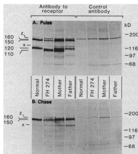
Fig. 8. Electrophoresis of LDL receptors immunoprecipitated from 35 S-labeled fibroblasts from FH 274 and his parents. Fibroblasts were cultured for 6 days and induced for synthesis of LDL receptors by incubation in lipoprotein-deficient serum for 16 hours (4). Cells were pulse-labeled with [ 35 S]methionine (140 \mu Ci/ml) (4) for 2 hours at 37°C, and isotopically labeled LDL receptors were solubilized either immediately (A) or 2 hours after the addition (chase) of unlabeled methionine (B). Cell monolayers were washed once with phosphate-buffered saline at 4°C, and detergent extracts were prepared and incubated with immune complexes (4) containing either monoclonal antibody to LDL receptor (IgG-C7) or a control monoclonal antibody (IgG-2001) (4). The incubation mixtures were layered onto multistep sucrose gradients, and the immunoprecipitates were collected by centrifugation and washed (4). The precipitates were dissolved by heating to 90°C for 5 minutes in buffer containing 10 percent (by volume) glycerol, 0.2M dithiothreitol, 2.3 percent (weight to volume) SDS, and 75 mM tris-chloride at pH 6.8 and subjected to SDS electrophoresis on 7 percent polyacrylamide gels, followed by autoradiography (4). The gels were exposed to x-ray film for 2 days. Apparent molecular sizes of the 35 S-labeled proteins were calculated from the position of migration of the following standards as determined by Coomassie blue staining: myosin (200 kD), \beta -galactosidase (116 kD), phosphorylase b (97 kD), and bovine serum albumin (68 kD). Band z is a protein that appears in control immunoprecipitations and is not related to the LDL receptor; band x is a proteolytic fragment of the receptor.
