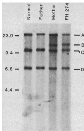
Fig. 2. Blot hybridization of Xba I-cleaved genomic DNA from FH 274 and his parents. Genomic DNA (5 \mu g) isolated from cultured fibroblasts from the indicated subject was digested with Xba I, subjected to electrophoresis, transferred to nitrocellulose, and hybridized with ^{32} P-labeled probe 1 (see legend to Fig. 1). The four relevant Xba I restriction fragments are designated A to D along the right side of the blot. Molecular size standards were generated by Hind III cleavage of bacteriophage \lambda DNA.
