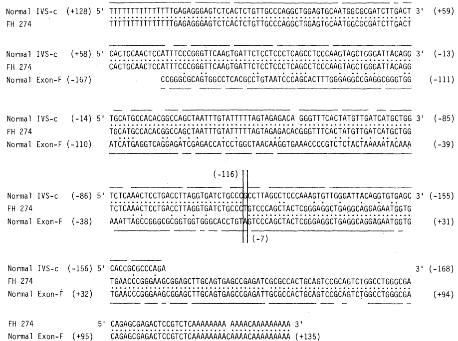
Fig. 5. Nucleotide sequences across the deletion joint in FH 274 and for the corresponding normal 5' and 3' DNA's. The normal and FH 274 sequence data were obtained as described in Fig. 4 and are numbered according to the scheme used for the consensus Alu sequence (11). The normal 5' sequence (top line), the sequence across the deletion joint in FH 274 (middle line), and normal 3' sequence (bottom line) are aligned with only two gaps of one base each. Dots between sequences indicate positions at which the sequences are identical. Horizontal lines above or below the normal sequence indicate positions at which the normal sequence is identical to the consensus Alu sequence (11). The two vertical lines at positions -116 and -7 denote the position of the deletion joint.
