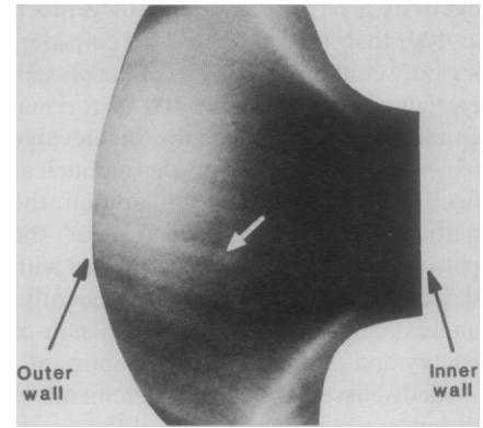
Fig. 4. Photograph of a plasma in the ASDEX tokamak at Garching, West Germany. The exposure time is 1/3000 second; thus fluctuations with frequencies less than 2 kHz are most prominent. The outline roughly corresponds to the profile of the minor cross section viewed in the direction tangential to the torus. The inner edge of the plasma is seen as the bright region curving along the inner wall. The filamentary structure in the photograph along the field lines (arrow) is due to the high level of turbulence near the plasma edge. [Photograph courtesy of D. H. J. Goodall (17)]
