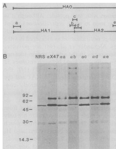
Fig. 2. Illustration of the power of sets of peptide antiserums used to track distinct regions of a protein simultaneously. (A) The influenza hemagglutinin precursor (HA0) and eventual products (HA1 and HA2). The synthetic peptides a to e, located within the HA0 sequence as shown (NH 2 - and COOH-terminal, flanking and spanning the HA1-HA2 junction), were coupled to a carrier and used to immunize rabbits as described (5-7). (B) The resulting antiserums ( \alpha a, \alpha b, \alpha c, \alpha d, \alpha e) and a positive control serum (antibody to X47 influenza virus, \alpha X47) and a negative control serum (normal rabbit serum, NRS) were used to precipitate extracts of [ 35 S]methionine-labeled influenza X47 virus-infected cells. The five antiserums to the peptides and \alpha X47 precipitated the HA0 molecule (this precursor is not appreciably cleaved during infection of cell lines), whereas the other precipitated proteins were nonspecific (sticky) since they also appeared in the normal control lane.
