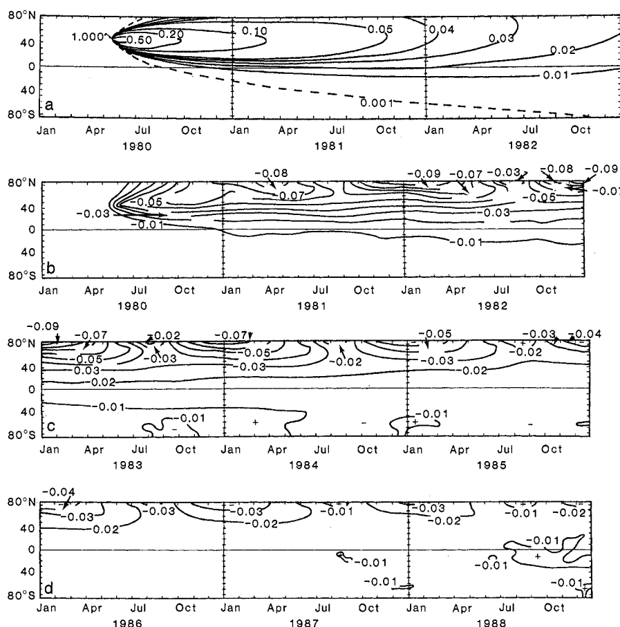
Fig. 1. (a) Relative concentration of volcanic dust from Mount St. Helens per 10^{\circ} latitude band assumed as forcing for climate model. (b to d) Surface temperature difference (degrees Celsius) between control run and climate model simulation using the forcing in (a) with interactive snow and ice.
