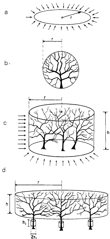
Fig. 4. A comparison of four boundary defense models for Oecophylla . (a) The two-dimensional model is that analyzed in the text. Its territory is circular with radius r . In three-dimensional models we have to consider several possibilities. (b) "Spheroid" is a spherical territory with radius r . This is appropriate to thick canopy systems in which the colony can expand outward from the queen nest in all directions for significant distances. (c) "Cylindrical 1" is a cylindrical territory of radius r and height h . All boundaries are defended and challenges come over the cylinder surface (arrows) but not the end faces, which are contained within the territory. (d) "Cylindrical 2," only the trunk surfaces leading up into the occupied canopy are defended. Trunk radius is r_1 and the defense occurs along a length h_1 of the trunks.
