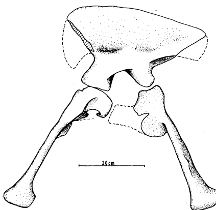
Fig. 1. Lateral view of the pelvis of Piatnitzkysaurus floresii n.g.n.sp. (new genus, new species), a megalosaurid carnosaur from the Jurassic of Patagonia (specimen PVL 4073).
