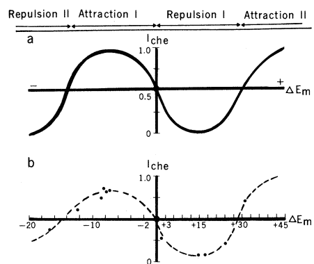
Fig. 2. (a) Graphical description of membrane potential control of chemokinesis. Change of membrane potential ( \Delta E_m ) from control (at origin) is plotted against the index of chemokinesis; I_{che} > 0.5 indicates attraction; < 0.5 indicates repulsion (see Table 1 legend). As chemical stimuli change E_m relative to control, animals will be attracted or repelled, depending on the magnitude and direction of the E_m change. (b) Data from Tables 1 and 2 plotted as \Delta E_m produced by the attractant or repellents versus I_{che} . Scale of \Delta E_m is different for depolarizing and hyperpolarizing stimuli.
