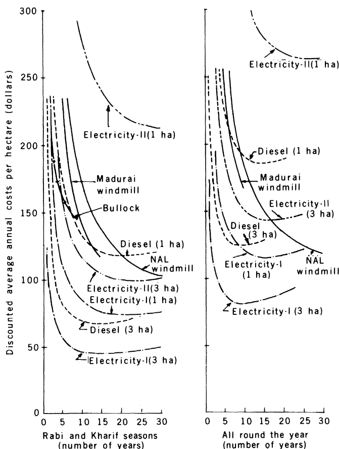
Fig. 2. Discounted average annual costs for irrigating 1 ha (under wheat or equivalent water-consuming crops) from open wells with an average depth of 6.67 m for the water table. Windmills would prove to be economical if they were designed to operate effectively at low wind speeds, and especially if they were utilized all year round.
