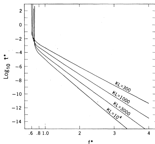
Fig. 8. The time for detachment, t^* = k_{-1} , is shown as a function of the force f^* = fr_0/kt \ln(KN_0) . Values of t^* were computed numerically, but Eq. 22 is a good approximation for f^* \geq 1.0 .
