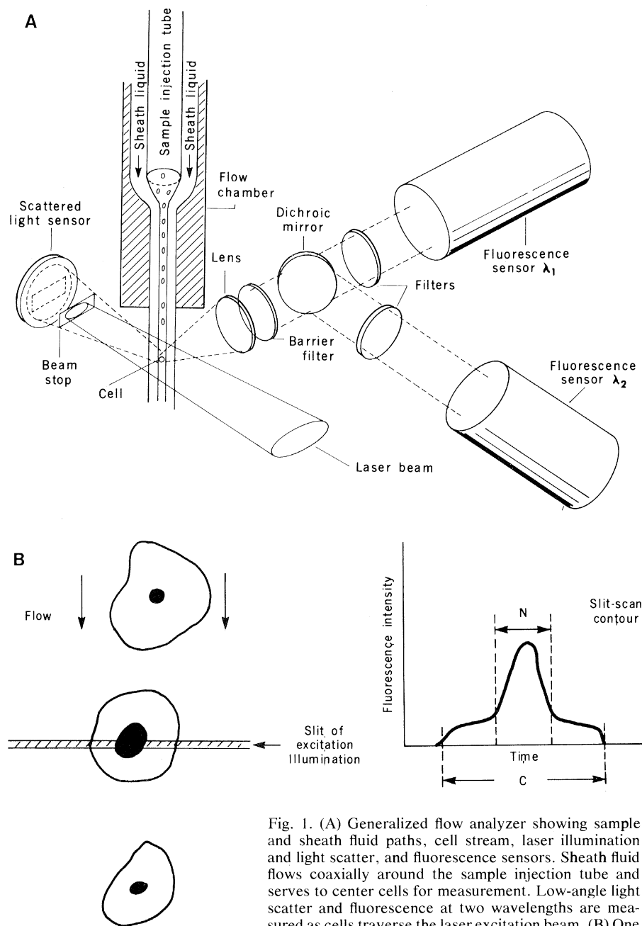
Fig. 1. (A) Generalized flow analyzer showing sample and sheath fluid paths, cell stream, laser illumination and light scatter, and fluorescence sensors. Sheath fluid flows coaxially around the sample injection tube and serves to center cells for measurement. Low-angle light scatter and fluorescence at two wavelengths are measured as cells traverse the laser excitation beam. (B) One-dimensional slit-scanning. Cells are sequentially illuminated as they flow through a slit of laser excitation illumination. Measurement of fluorescence from the cell at discrete time intervals yields a fluorescence contour. Contours may be analyzed to provide cell diameter (C), nuclear diameter (N), nuclear to cell diameter ratio, nuclear fluorescence, cytoplasmic fluorescence, and certain other low-resolution morphological information.
