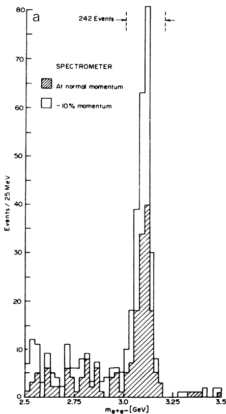
Fig. 12. (a) Mass spectrum for events in the mass range 2.5 < m_{ee} < 3.5 \text{ GeV}/c^2 . Shaded events correspond to those taken at the normal magnet setting; unshaded ones correspond to a spectrometer magnet setting 10 percent lower than the normal value. (b) Measurement of the width of the J. The width is shown to be less than 5 MeV.
