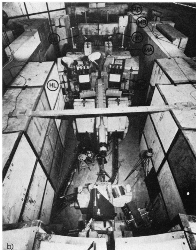
Fig. 1. (a) Plan view of the spectrometer: MD , MA , and MB , dipole magnets; L1 to L4 and R1 to R4 , triggering counters; LC , RC , HL , and HR , large-aperture threshold Čerenkov counters; SLC and SRC , shower counters; TL , QL , VL , TR , QR , and VR , are hodoscopes; and QM , quantameter. (b) Overall view of my first experiment at DESY. The positions of LC , RC , HL , HR , MA , and MD are all marked. The physicist on the left is Dr. A. J. S. Smith; on the right is Dr. C. L. Jordan.
