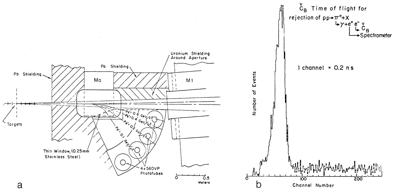
Fig. 10. Measurement of e^+e^- from \pi^0 \rightarrow \gamma + e^+ + e^- decay. (a) Side view of magnet M_0 , which bends the various low-energy trajectories ( P_e ) of e^\pm into C_B . (b) Relative timing between an electron pulse from C_B and a positron trigger from the main spectrometer arm or vice versa.
