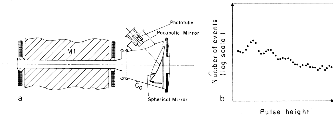
Fig. 7. (a) Plan view of the C_0 counter shown in its location in the experiment. (b) Pulse-height spectrum from the phototube (RCA C31000M) of the C_0 Čerenkov counter with helium as radiator. Clearly visible are the one, two, and three photoelectron peaks.
