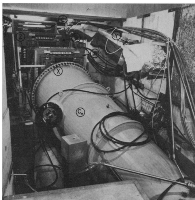
Fig. 8 (left). Overall view of the detector. Fig. 9 (right). End view of one arm, showing part of the Čerenkov counter C_e and the chambers A, B, C, with part of the 8000 amplifiers X, cables Y, and hodoscopes Z. The lead-glass counter is at the end of chamber U.
