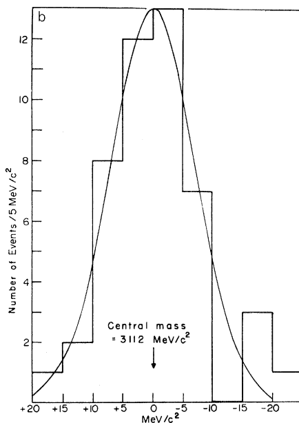
Fig. 12. (a) Mass spectrum for events in the mass range 2.5 < m_{ee} < 3.5 \text{ GeV}/c^2 . Shaded events correspond to those taken at the normal magnet setting; unshaded ones correspond to a spectrometer magnet setting 10 percent lower than the normal value. (b) Measurement of the width of the J. The width is shown to be less than 5 MeV.
