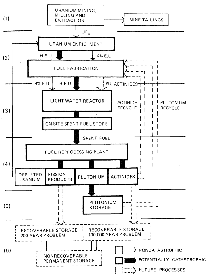
Fig. 3. The light water fuel cycle, showing portions currently operational and non-operational in the United States. The abbreviations E.U. and H.E.U. stand for enriched and highly enriched uranium, respectively.
