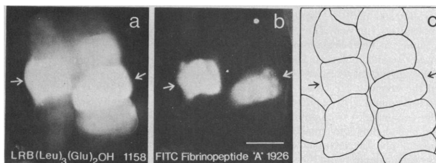
Fig. 1. Probing junctional membrane channels with two molecules close to the size limit of permeation. The red fluorescent tracer LRB(Leu) 3 (Glu) 2 OH (1158 daltons), the largest permeant molecule of the present series, is injected into the cells marked with an arrow, together with the yellow-green fluorescent tracer FITC-fibrinopeptide A (1926 daltons). (a) Distribution of the red tracer (1158 daltons) photographed (darkfield) in black and white 40 minutes after injection. (b) Distribution of the yellow-green tracer (1926 daltons) 45 minutes after injection. (The two fluorescences are set apart by the use of different excitation wavelengths and barrier filters.) The red tracer spread from the injected cells to several neighbors; the yellow-green tracer stayed within the injected cells (calibration bar, 100 μm).
