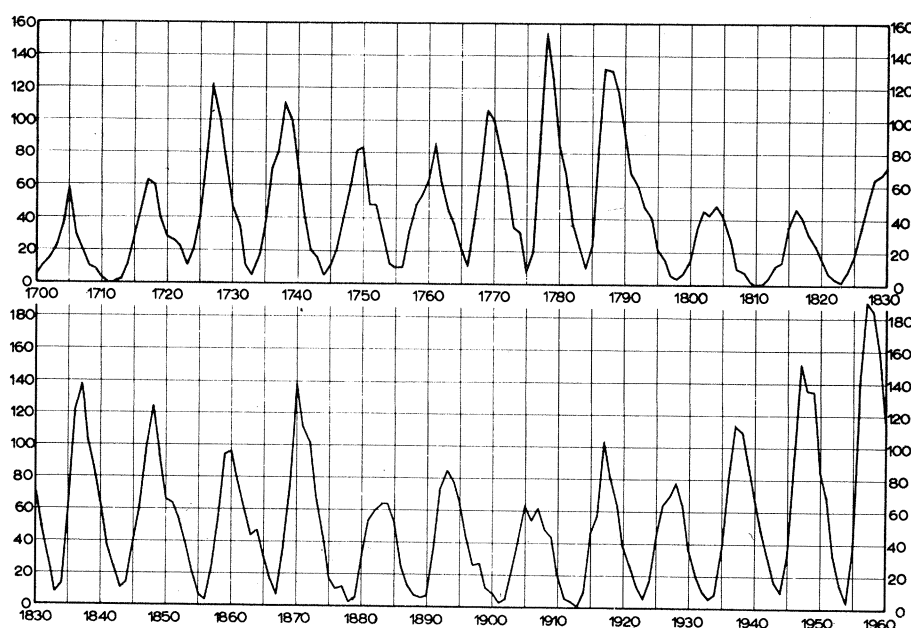
Fig. 1. Annual mean sunspot number, R , from 1700 to 1960. [From (3); courtesy of M. Waldmeier]
