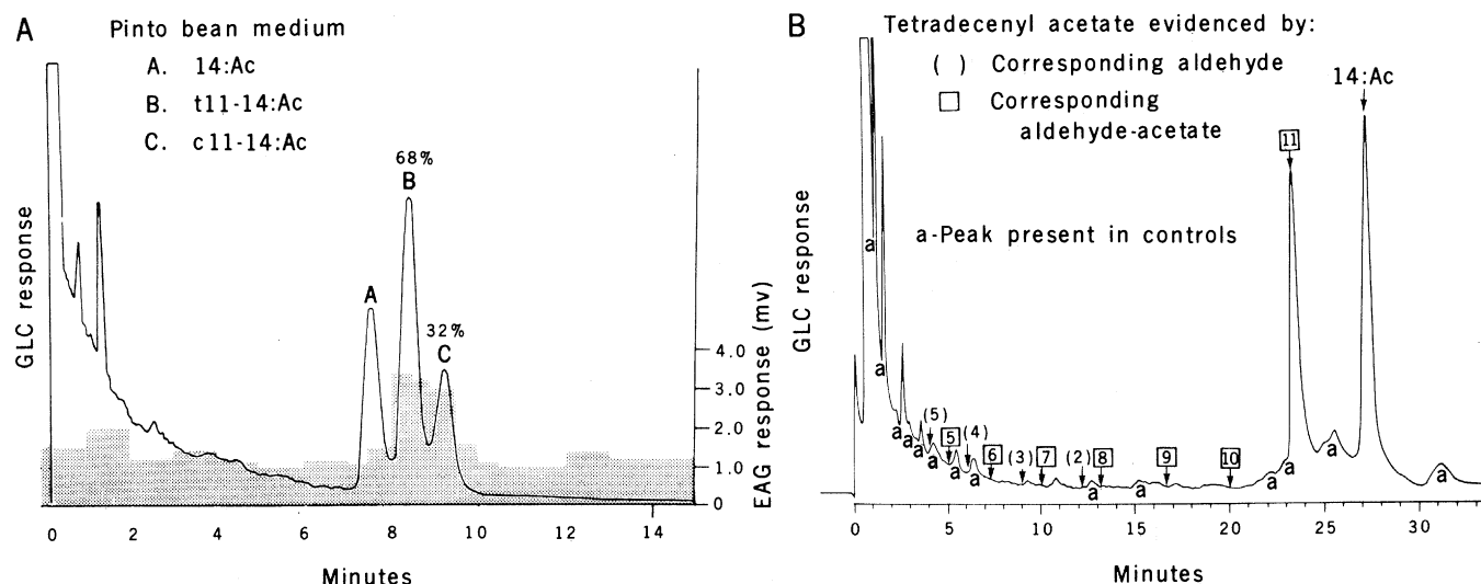
Fig. 1. (A) Tip extract from A. semiferanus females reared on pinto bean medium fractionated on an XF-1150 column at 154°C. The GLC tracing of crude extract and the EAG response (shading) to the 14-carbon acetates from crude tip extract collected from OV-1 are shown. (B) GLC tracing (OV-1) of microozonolysis products of the 14-carbon acetates from crude tip extract collected from OV-1.
