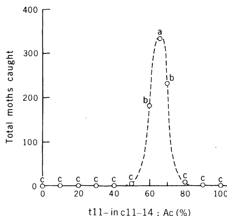
Fig. 2. Trap catches of A. semiferranus males with varying ratios of t11-, and c11-14 : Ac. This test was conducted from 6 to 16 July 1975 using Sectar traps spaced 15 to 20 m apart. The six replicates were rerandomized each day between 8 and 11 July. Means for the treatments marked by the same letter were not significantly different at the 5 percent level.
