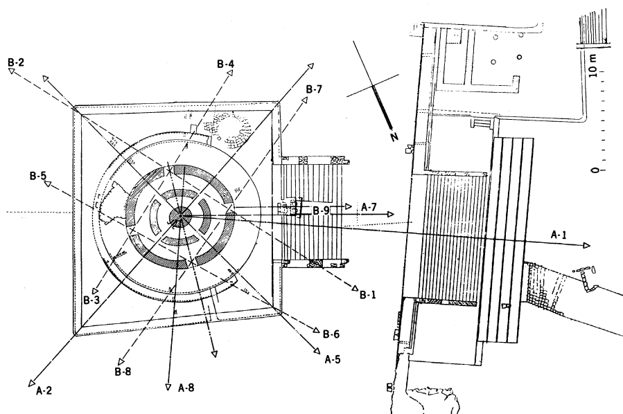
Fig. 5. Plan of the upper platform and stairway of the lower platform of the Caracol as it appears at present, showing alignments measured by the authors.
