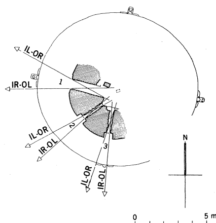
Fig. 6. Sketch of horizontal cross section through the Caracol windows showing windows labeled 1, 2, and 3 and the pairs of diagonal sight lines.
