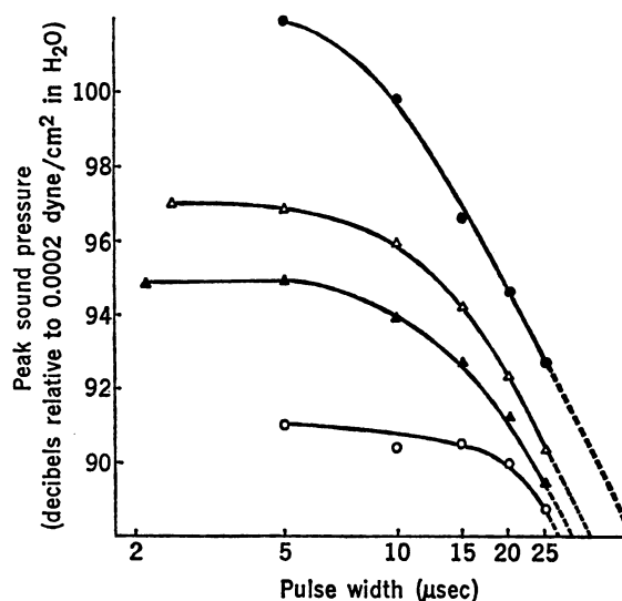
Fig. 2. The peak sound pressure of the microwave-generated acoustic transient, as a function of the microwave pulse width and filter bandwidth. Filter bandwidth: ●, 200 hertz to 60 khz; △, 200 hertz to 40 khz; ▲, 200 hertz to 30 khz; ○, 200 hertz to 20 khz. The 0.15N KCl solution was in a large rectangular expanded polystyrene tank, at 25°C. The sound pressures were increased by 2.9 db to simulate measurements at 37°C. The dotted lines indicate the function P_0 \propto I_0 (Eq. 1). This figure shows that, for short pulses, P_0 \propto I_0 \tau , in agreement with psychophysical observations of the microwave "hearing" effect. The microwave intensity was adjusted so that the incident energy density per pulse was 80 \mu J/cm 2 , the threshold for microwave "hearing" in an average subject.
