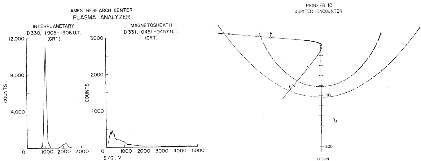
Fig. 1 (left). Comparison of the solar wind ion spectra taken upstream and downstream from Jupiter's bow shock for the inbound portion of the Pioneer 10 Jupiter flyby. Fig. 2 (right). Projection of the Pioneer 10 encounter trajectory onto Jupiter's orbital plane, with the shape and location of the bow shock and magnetopause scaled from the case at Earth. The crosses along the trajectory show the locations of various shock and magnetopause observations during the Pioneer 10 Jupiter flyby, where E/Q is energy per unit charge in volts.
