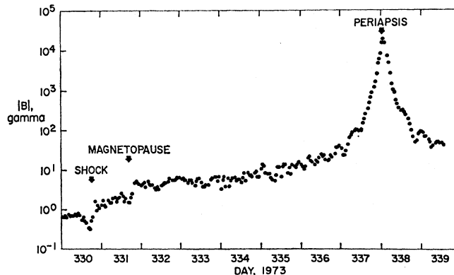
Fig. 1. Pioneer 10 encounter: Jovian field magnitude. One-hour averages of the field magnitude, |B| , are shown for 7 days from the bow shock crossing inbound to periapsis and for 2 days outbound.
