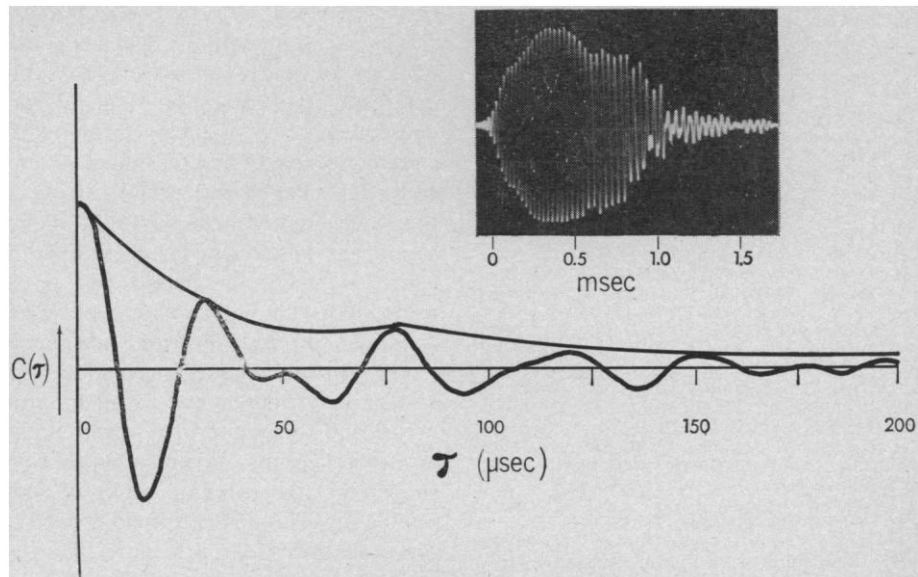
Fig. 4. The autocorrelation function of an Eptesicus sonar cry for time-delay differences up to 200 \mu sec, showing the upper envelope of the function. (Inset) The oscilloscope trace of the cry itself. The envelope of the autocorrelation function represents the ambiguity in echo arrival time (target range) confronting the bat when it processes the echoes of its cries.
