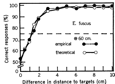
Fig. 2. The average performance of three Eptesicus in discriminating differences of target range (empirical curve), and the performance predicted from the autocorrelation function of the Eptesicus sonar cry (theoretical curve).
