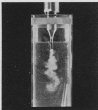
½" Ultratip cavitating oil in a glass pipe.
