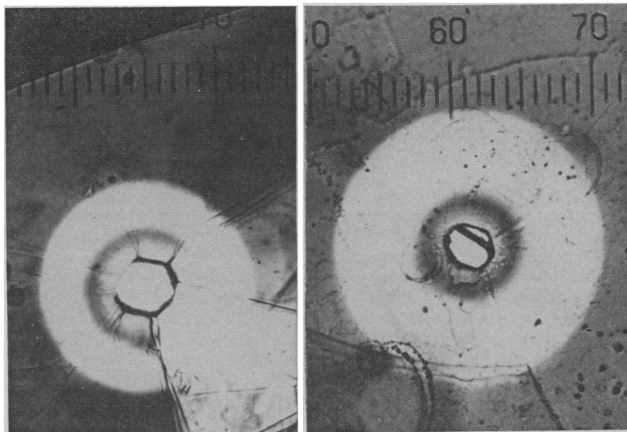
Fig. 2 (left). A giant halo approximately 57 \mu\text{m} in radius, presumably due to the long-range alpha particles from \text{Po}^{212} ( E = 10.55 MeV). One scale division = 10 \mu\text{m} . Fig. 3 (right). A giant halo approximately 84 \mu\text{m} in radius, whose origin is unknown. If the halo is due to long-range alpha particles, the energy would be about 13.1 MeV. One scale division = 10 \mu\text{m} .
