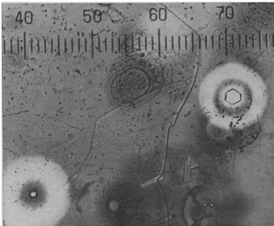
Fig 1. The halo on the right is a combination uranium and thorium halo, with the inner ring radius of 34 \mu\text{m} from the uranium daughter emitter \text{Po}^{214} ( E = 7.68 \text{ Mev} ) and the outer ring radius of 40 \mu\text{m} from the thorium daughter emitter \text{Po}^{212} ( E = 8.78 \text{ Mev} ). The halo on the left with a relatively small inclusion is a giant halo with about a 50- \mu\text{m} radius. One scale division = 10 \mu\text{m} .
