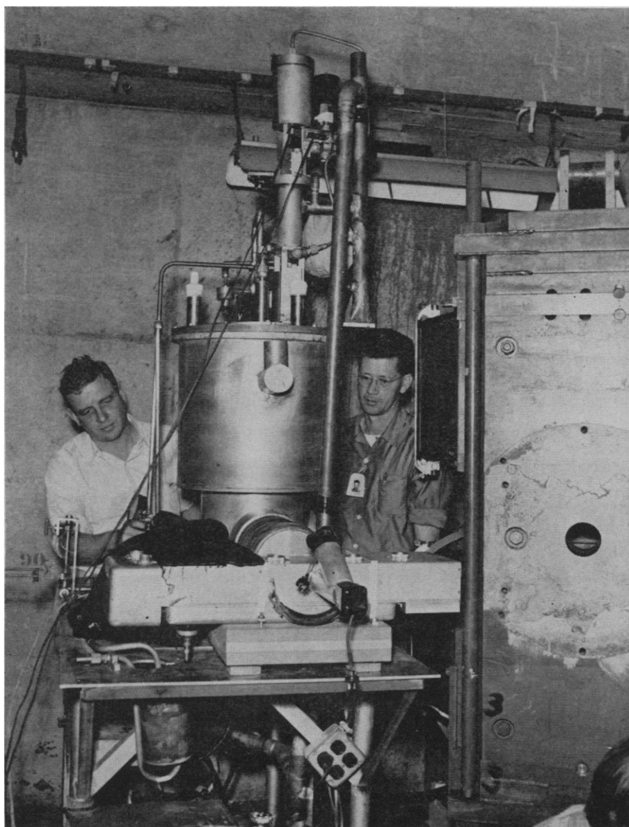
Fig. 4. Four-inch chamber. D. Parmentier (left) and A. J. Schwemin (right).
