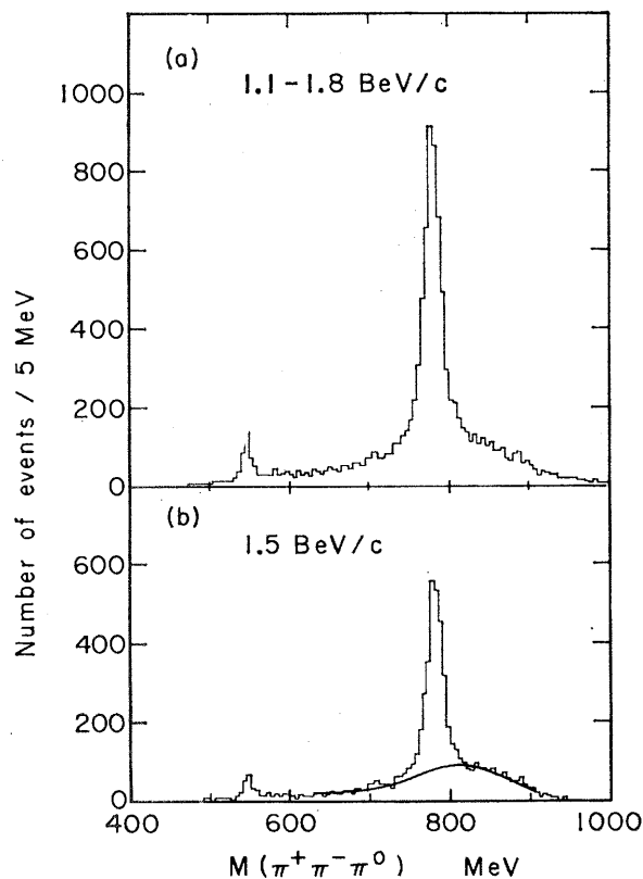
Fig. 18 (left). Discovery of the \omega meson.
