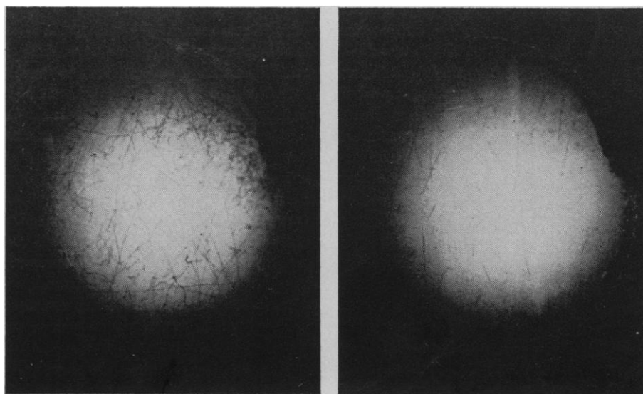
Fig. 3. Tracks in 2.5-inch bubble chamber. (Left) Neutrons; (right) gamma rays.
