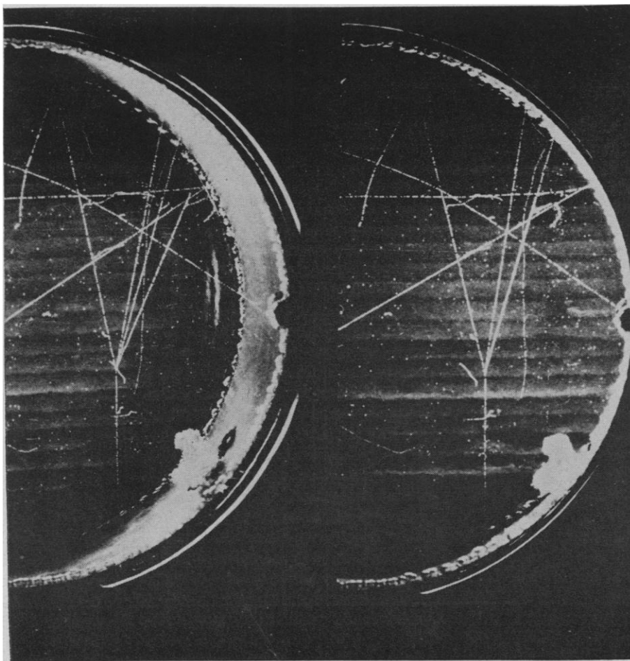
Fig. 6. Multiple meson production in 4-inch bubble chamber.
