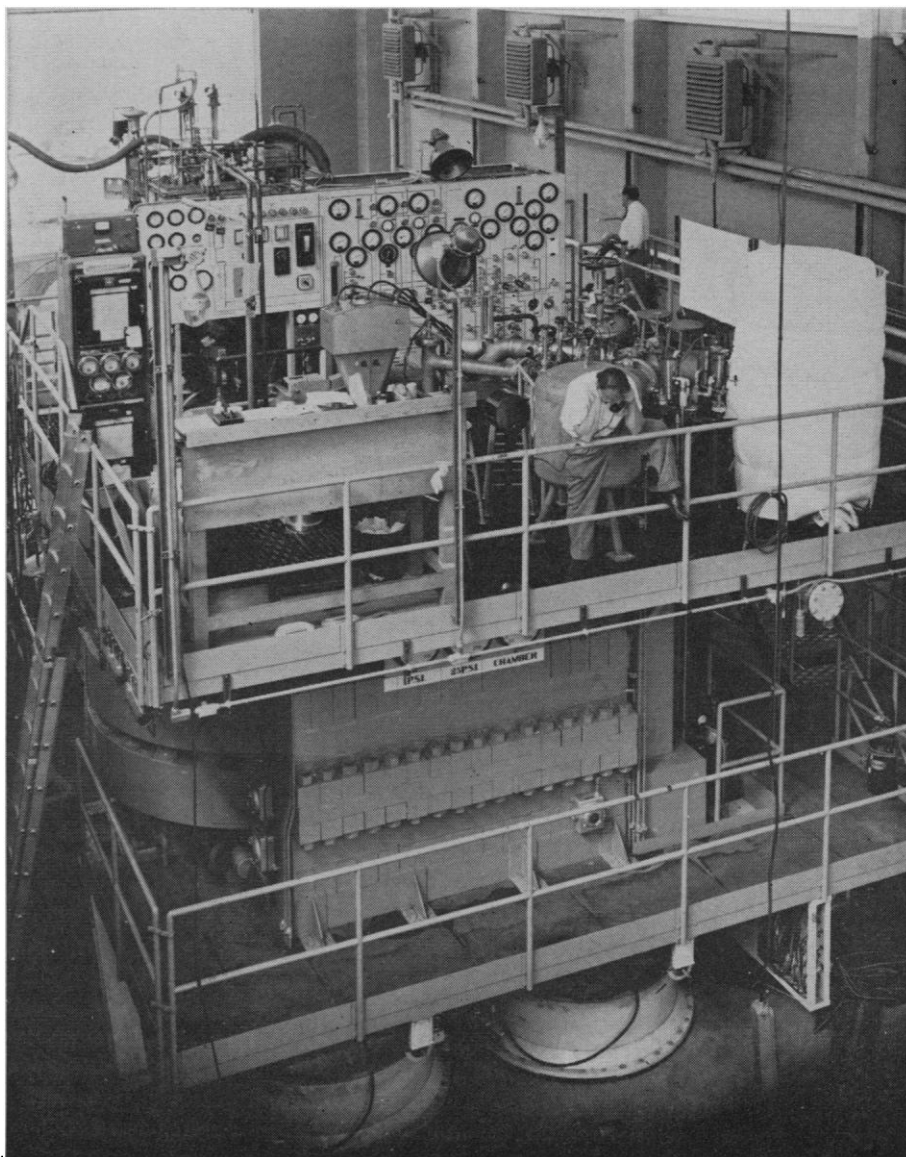
Fig. 7. Seventy-two-inch bubble chamber in its building.
