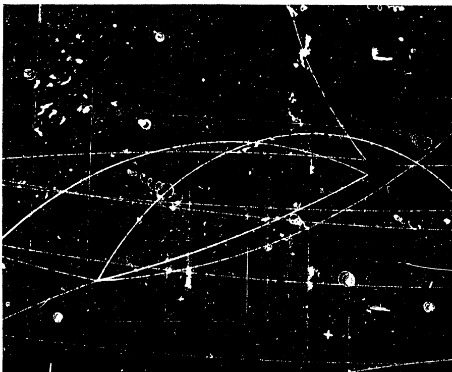
Fig. 17. First production of antilambda.
