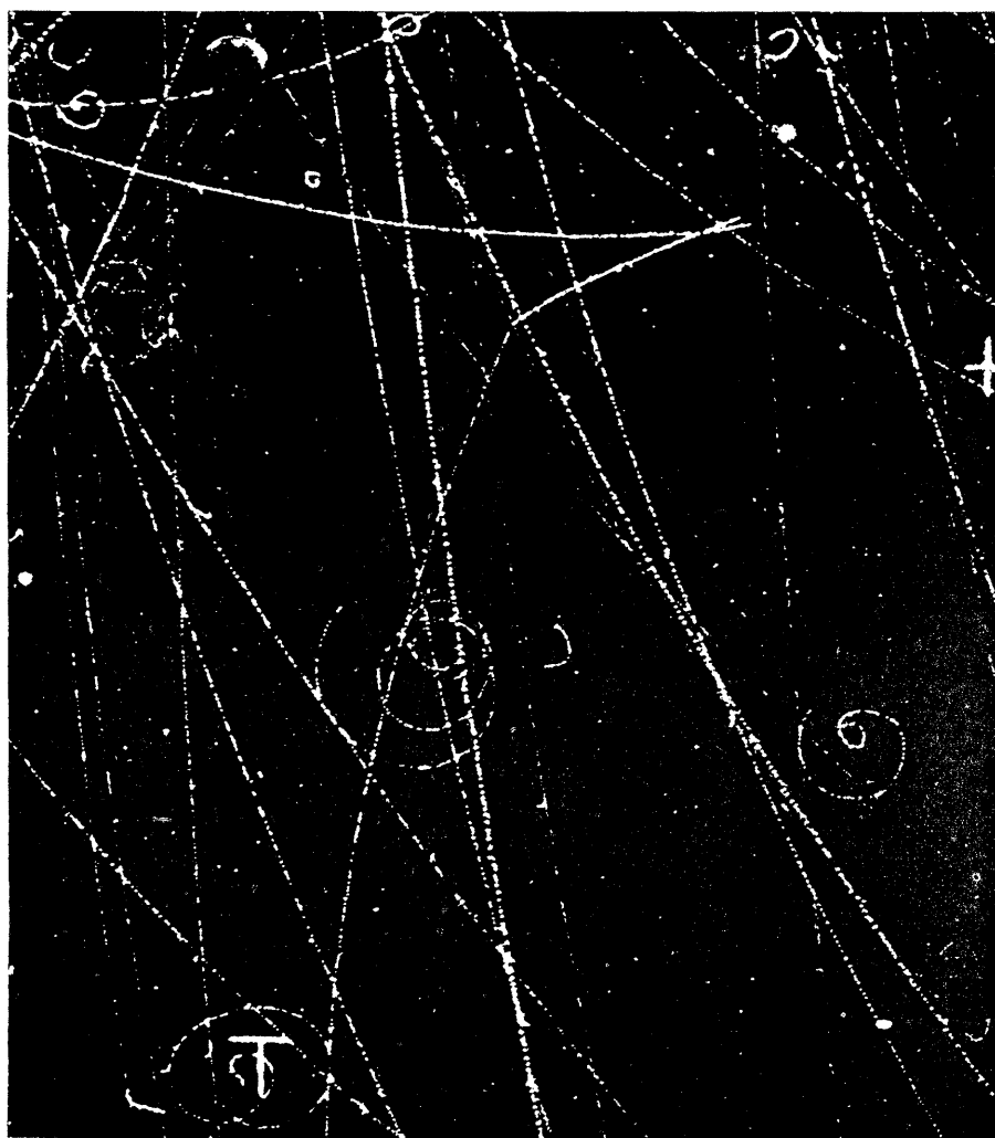
Fig. 10. Muon catalysis (with gap).
