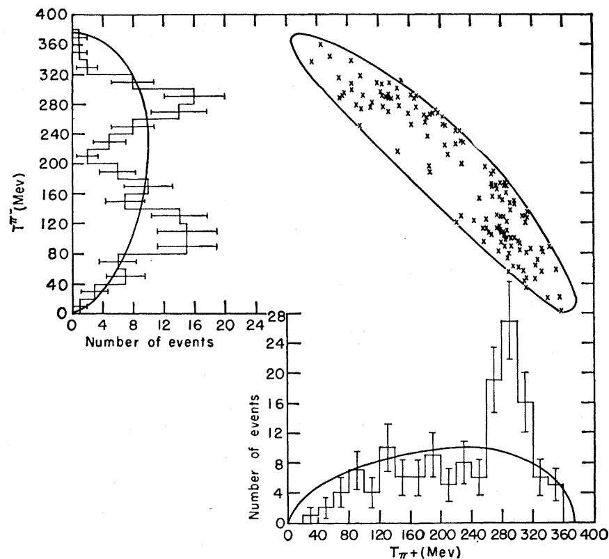
Fig. 13. Discovery of the Y_1^*(1385) .
