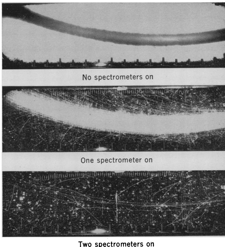
Fig. 11. Separated beam in 72-inch bubble chamber.
