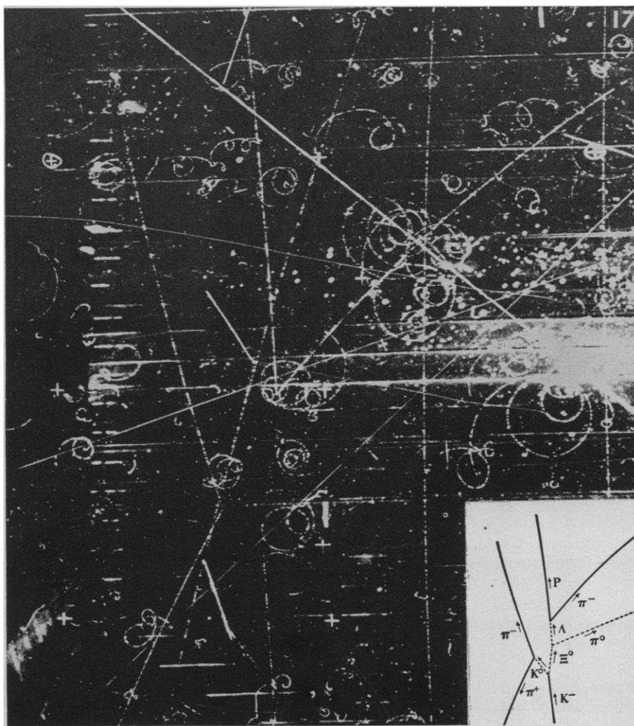
Fig. 12. Production and decay of a neutral cascade hyperon ( \Xi^0 ).
