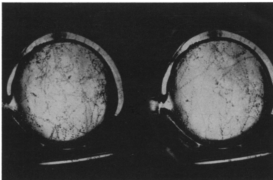
Fig. 2. First tracks in hydrogen.
