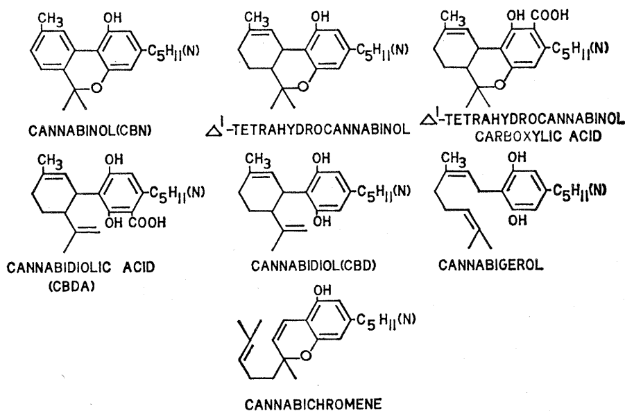
Fig. 2. Structures of major constituents of hashish.
