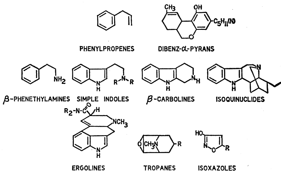
Fig. 1. Chemical structures of various types of hallucinogens.
