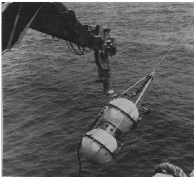
Fig. 2 (left). Instrument capsule is hoisted overboard for free fall to the sea floor. Fig. 3 (right). Instrument support frame with various components identified in Fig. 1. The ballast is attached by a bolt (0.375 inch in diameter) at the bottom of the frame. Electrical connections to batteries are made through connectors at base.
