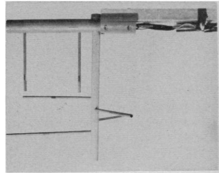
Fig. 5. The Caldwell water velocity probes. Copper fittings at the center of Micarta tubes contain an indirectly heated thermistor. The temperature of the copper element is dependent upon the cooling of water. The vertical pair of probes provides measurement of water speed parallel to the bottom. Two pairs of 90° horizontally mounted probes provide data on current direction.
