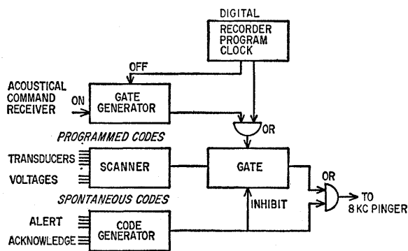
Fig. 8 (left). Pinger system of the capsule provides programmed or commanded instrument checks to monitor five transducers and three battery voltages. Spontaneous codes are automatically transmitted to alert the ship to serious difficulty or to acknowledge commands transmitted by the ship. Fig. 9 (right). Spontaneous pinger codes provide a method for distinguishing any single code or any combination of codes. The number of pulses in a group is equal to the sum groups in the individual codes. The combination of c and d results in a 12-pulse sequence formed by combination of the four-pulse c code with the eight-pulse d code. Addition of an acknowledge code produces groups of triple pings for approximately 30 seconds.
