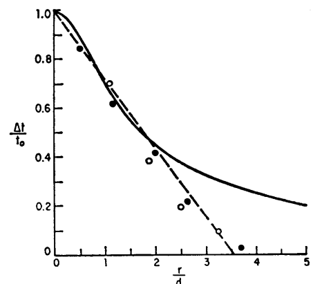
Fig. 12. If we assume unrefracted acoustic paths, the range, r , of the capsule on the bottom can be calculated from measurements for surface echo time delay, \Delta t , if the hydrophone depth, h , water depth, d , and sound velocity, v , are known. The unrefracted path assumption (solid line) matches data obtained at sea only for r < 2d ; a linear approximation to the data (dashed line) is adequate for navigating the ship.
