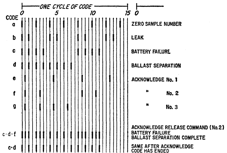
Fig. 8 (left). Pinger system of the capsule provides programmed or commanded instrument checks to monitor five transducers and three battery voltages. Spontaneous codes are automatically transmitted to alert the ship to serious difficulty or to acknowledge commands transmitted by the ship. Fig. 9 (right). Spontaneous pinger codes provide a method for distinguishing any single code or any combination of codes. The number of pulses in a group is equal to the sum groups in the individual codes. The combination of c and d results in a 12-pulse sequence formed by combination of the four-pulse c code with the eight-pulse d code. Addition of an acknowledge code produces groups of triple pings for approximately 30 seconds.
