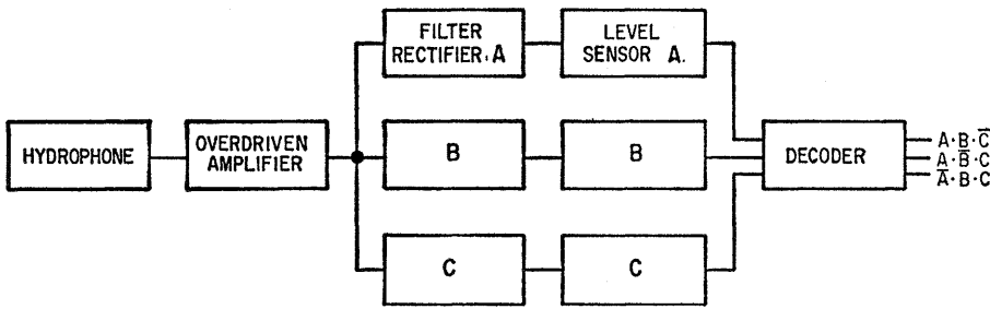
Fig. 7. Command receiver of the capsule decodes acoustical signals sensed by the hydrophone. After amplification the output filters A, B, and C are decoded. Output commands are activated whenever two of three frequencies are present and the third signal is absent.
