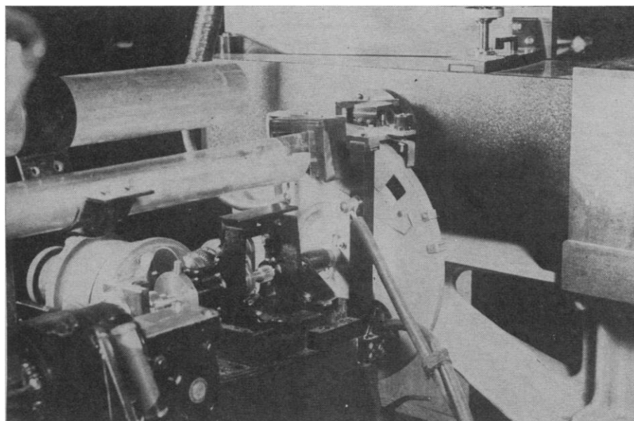
Fig. 1. Part of the original flash-photolysis apparatus showing the rotating sector with shutter and trigger contacts.
