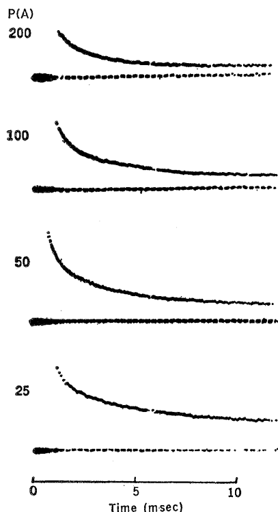
Fig. 4 (left). Oscillograph traces of I_2 absorption after flash photolysis of iodine in excess argon. P(A) is argon pressure in millimeters of mercury.
