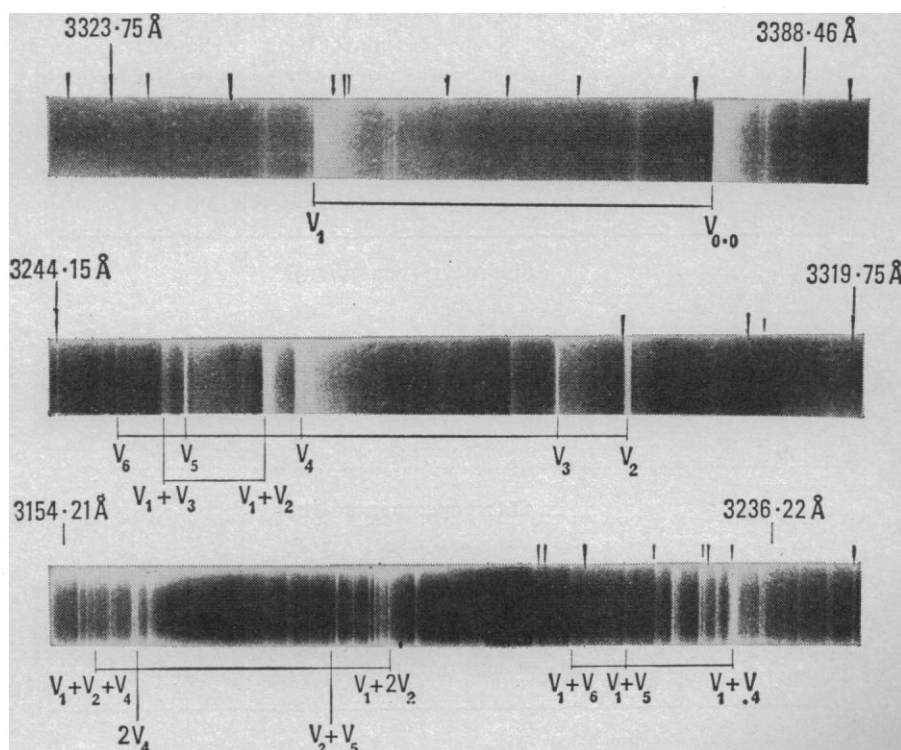
Fig. 10. Absorption spectrum of the cyclopentadienyl radical.
