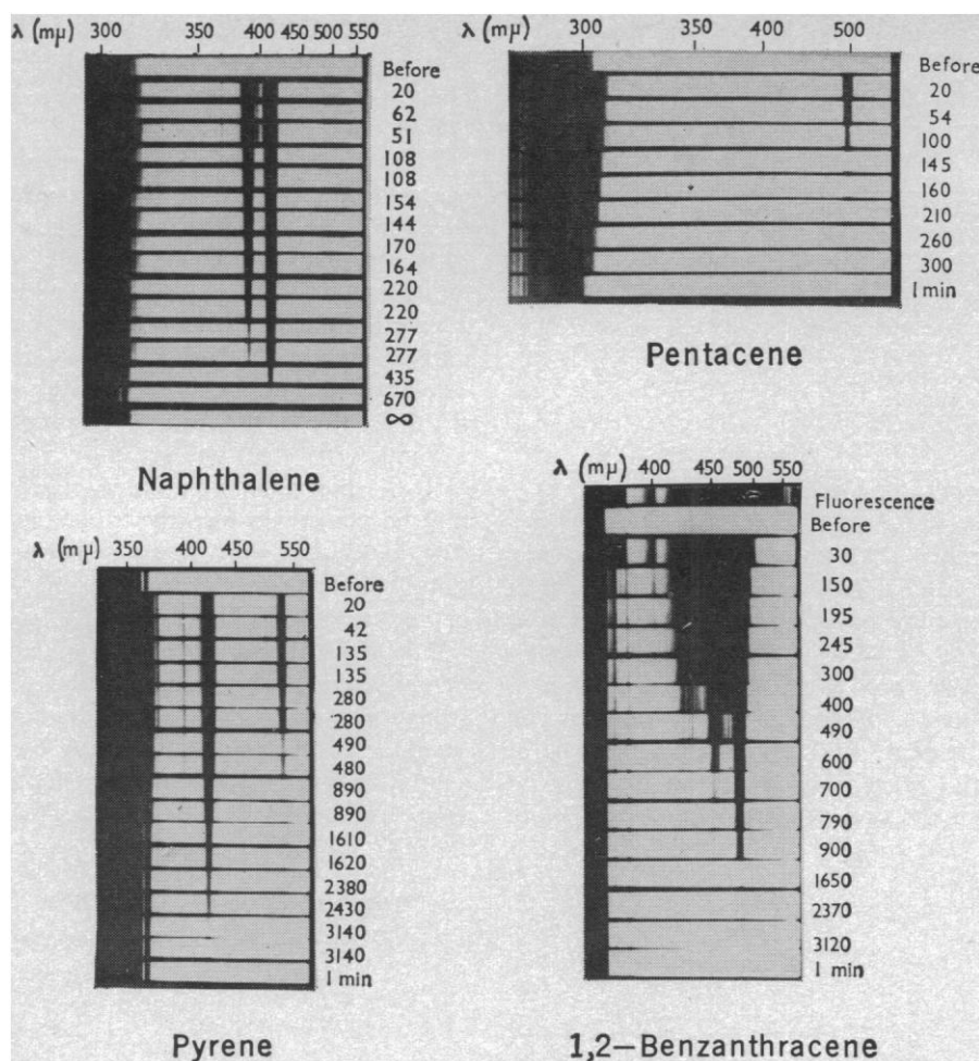
Fig. 15 (left). Sequences of spectra after flash photolysis of four aromatic hydrocarbons in solution showing formation and decay of their triplet states. Delays in microseconds.
