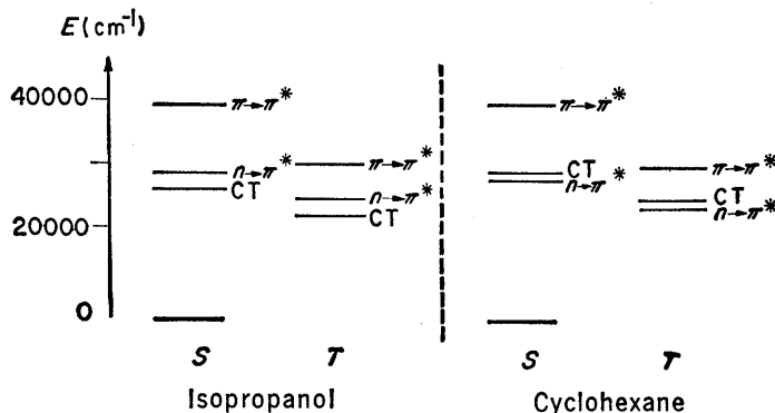
Fig. 17 (left). Optical density plot of triplet anthroic acid versus pH used to derive the triplet state acidity constant of this compound. Fig. 18 (right). Energy of singlet ( S ) and triplet ( T ) states of p -amino benzophenone in isopropanol and in cyclohexane. In isopropanol the lowest triplet is of charge transfer (CT) type and therefore no reaction occurs; in cyclohexane the lowest triplet is the reactive n-\pi^* type, and hydrogen abstraction occurs from cyclohexane to yield a ketyl radical.
