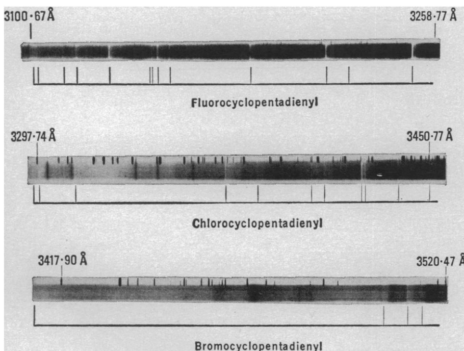
Fig. 11. Absorption spectra of three halogenated cyclopentadienyl radicals.
