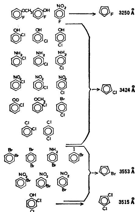
Fig. 12. Observed fission processes of benzene derivatives to form cyclopentadienyl radicals.
