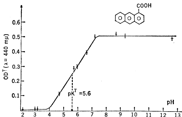
Fig. 17 (left). Optical density plot of triplet anthroic acid versus pH used to derive the triplet state acidity constant of this compound. Fig. 18 (right). Energy of singlet ( S ) and triplet ( T ) states of p -amino benzophenone in isopropanol and in cyclohexane. In isopropanol the lowest triplet is of charge transfer (CT) type and therefore no reaction occurs; in cyclohexane the lowest triplet is the reactive n-\pi^* type, and hydrogen abstraction occurs from cyclohexane to yield a ketyl radical.
