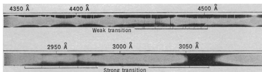
Fig. 6. Absorption spectrum of the benzyl radical in the vapor phase after flash photolysis of toluene. Path length = 8 m.
