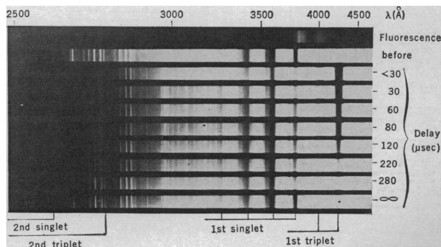
Fig. 13 (top right). Transitions involved in flash-photolysis studies of the triplet state. Fig. 14 (bottom right). Absorption spectra following flash photolysis of a solution of anthracene in hexane solution.
