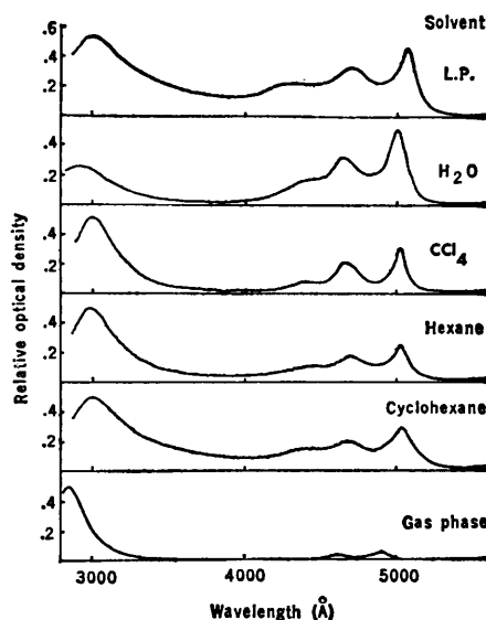
Fig. 7 (left). Absorption spectrum of the phenoxyl radical in the gas phase and in various solvents after flash photolysis of phenol.
