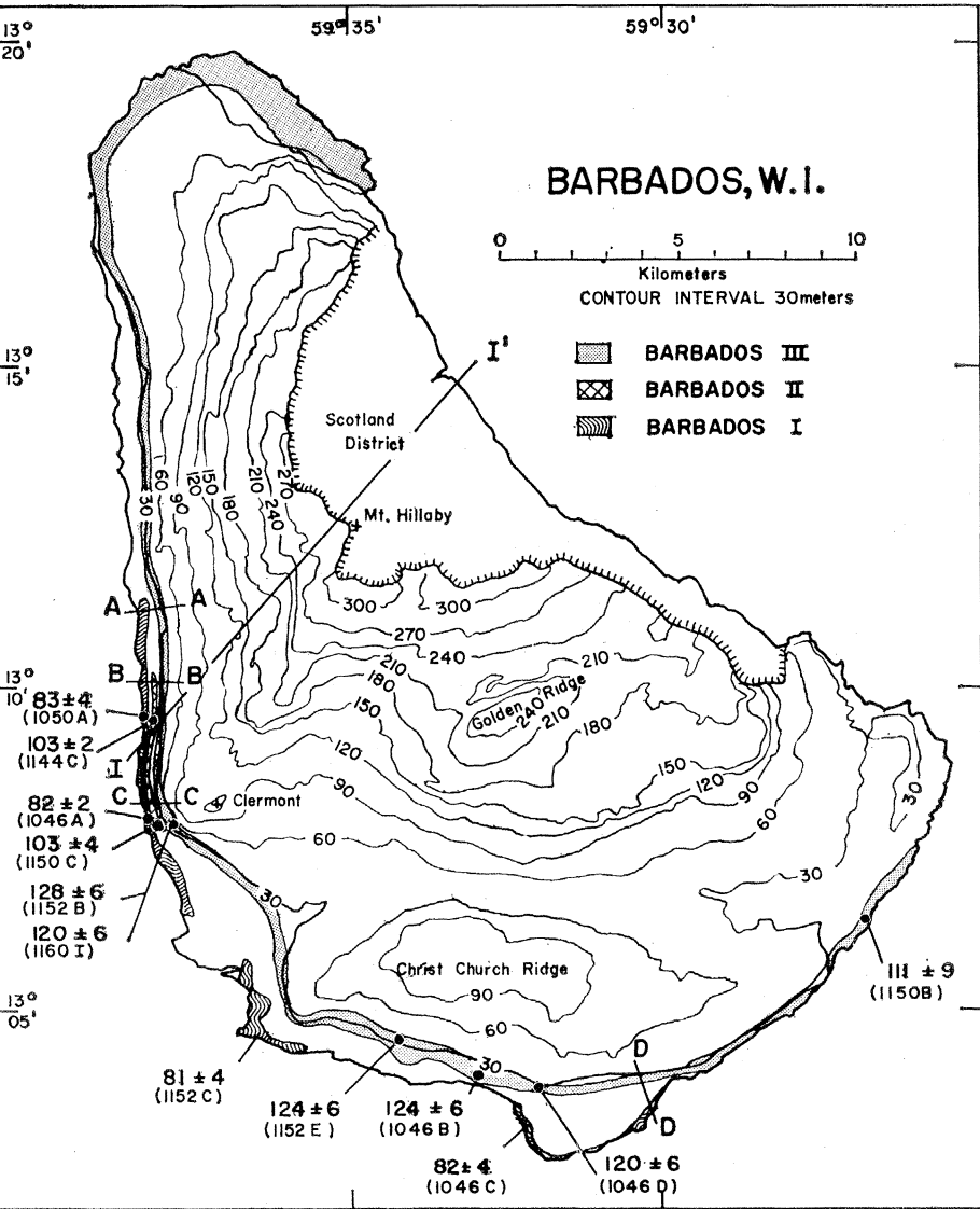
Fig. 1. General geology of Barbados, and topography of the coral cap. The three terraces discussed occur along the north, west, and south coasts of the island. Sources and ages ( \times 10^3 years) of samples listed in Table 1 are indicated. Letters A-D show the locations of traverses used in calculating the paleolevels of the sea (Table 3).
