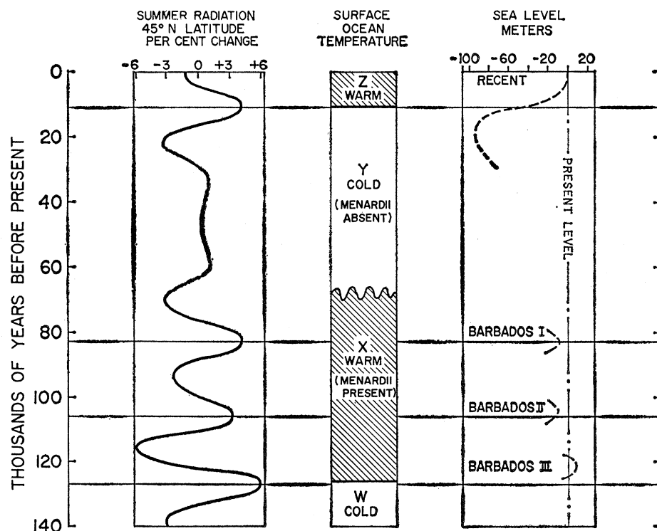
Fig. 2. Correlation of Broecker's (7) modified summer-insolation curve for the northern hemisphere with the ocean's surface-temperature record for Atlantic deep-sea cores, and with the record of fluctuations in sea level.
