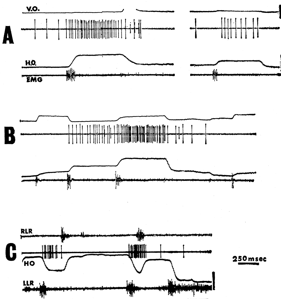
Fig. 1. Discharge of single antidromically activated units (A, B, C) recorded in different experiments from the frontal eye fields during eye movement. V.O., vertical oculogram; H.O., horizontal oculogram. Electromyographic record (EMG) from lateral rectus muscle on the right (RLR) and left (LLR) side. Vertical bars indicate 20° and 10° when related to H.O. and V.O.
