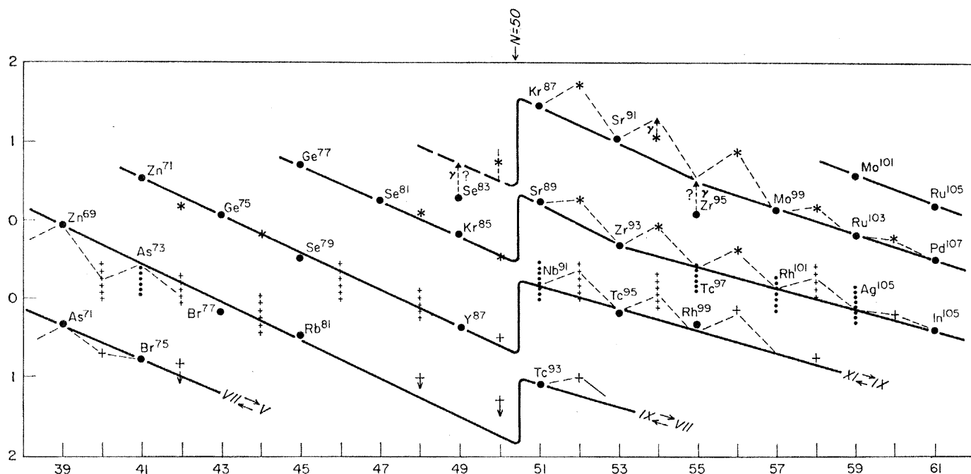
Fig. 2. Beta decay energies in the neighborhood of N = 50 .
