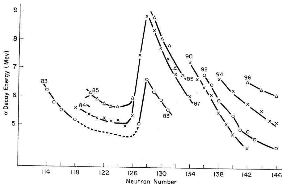
Fig. 3. Energy release in alpha decays. [After Seaborg and Perlman]
