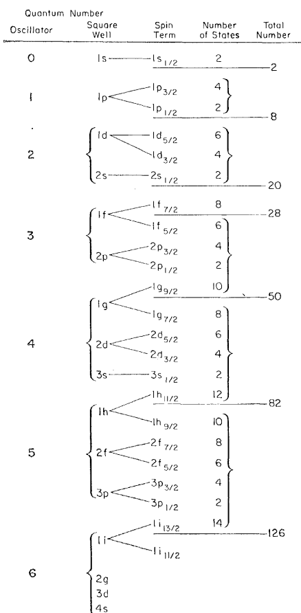
Fig. 5. Schematic level diagram.
