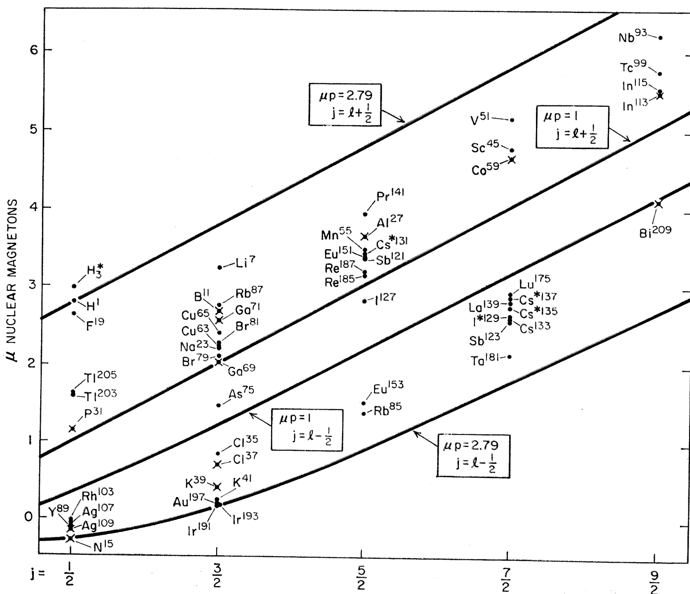
Fig. 7. Magnetic moments of nuclei with odd proton, even neutron number.
