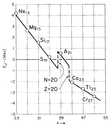
Fig. 1. Beta decay energies in the neighborhood of N = 20 .
