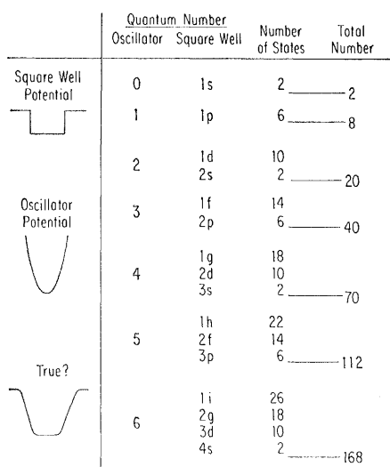
Fig. 4. Energy levels in a square well.
