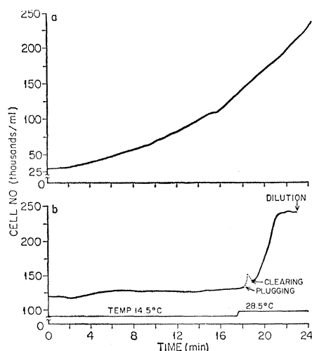
Fig. 2. Recordings of the changes in cell number over (a) a logarithmic growth period, and (b) a synchronous growth cycle of Astasia longa .
