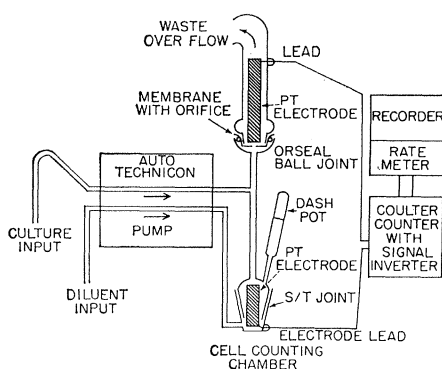
Fig. 1. Schematic diagram of the apparatus for the continuous recording of cell number, showing details of the counting chamber.
