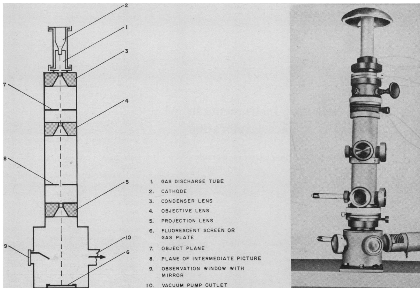
Fig. 2. The first supermicroscope, developed by E. Ruska in 1933. (Left) Functional diagram; (right) photograph.
