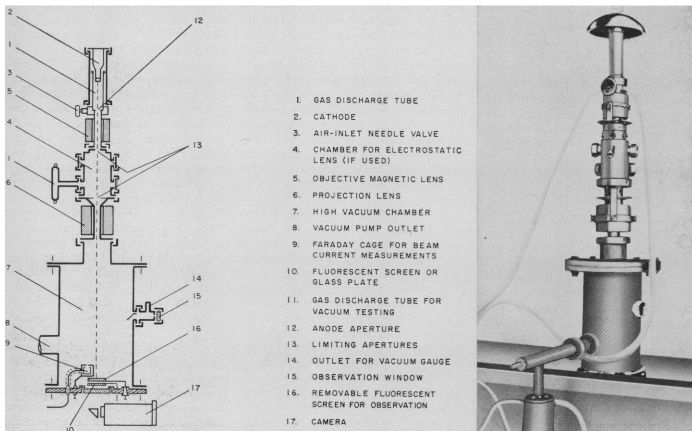
Fig. 1. The first electron microscope, developed by M. Knoll and E. Ruska in 1931. (Left) Functional diagram; (right) photograph.
