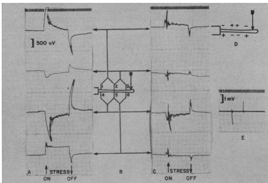
Fig. 1. Electrical response of amphibian bone (tibio-fibula of bullfrog) to bending stress. Electrode placements and connections on bone in clamp are shown schematically at B. Differential inputs were used and the center electrodes (Nos. 2 and 5) are common to two channels. The amplification for record C is the same as that shown for A, and upward deflection of the pen in both indicates a negative potential. The applied stress in A was 30 g, that of C was 15 g. Each mark at top of charts A and C equals 1 second. The potentials developed should be compared to those observed from a quartz piezo-electric crystal with the same instrumentation (E). The crystal produces brief potential changes in one direction on application of stress, and equally brief impulses of opposite polarity on release of stress. The potentials obtained from the bone are similar but decrement much more slowly and show a sustained potential during the time the stress is applied. This implies a persistent charge separation under stress with a charge distribution on the bone surface, as shown schematically at D.
