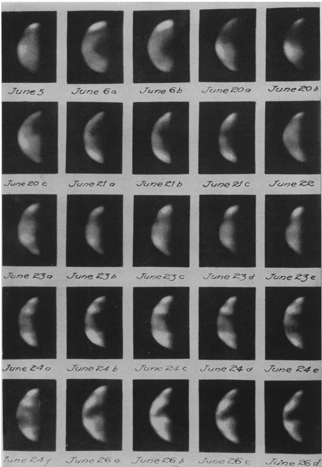
Fig. 2. Sequence of ultraviolet photographs of Venus taken with the 60- and 100-inch reflectors at Mount Wilson Observatory by F. E. Ross, in June and July 1927. [From Astrophys. J. 68 , 57 (1928), with permission from the University of Chicago Press. Copyright 1928 by the University of Chicago]
