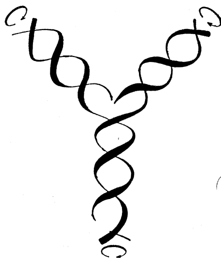
Fig. 2. The scheme of Watson and Crick for DNA replication. "Unwinding and replication proceed pari passu . All three arms of the Y rotate as indicated" (14).
