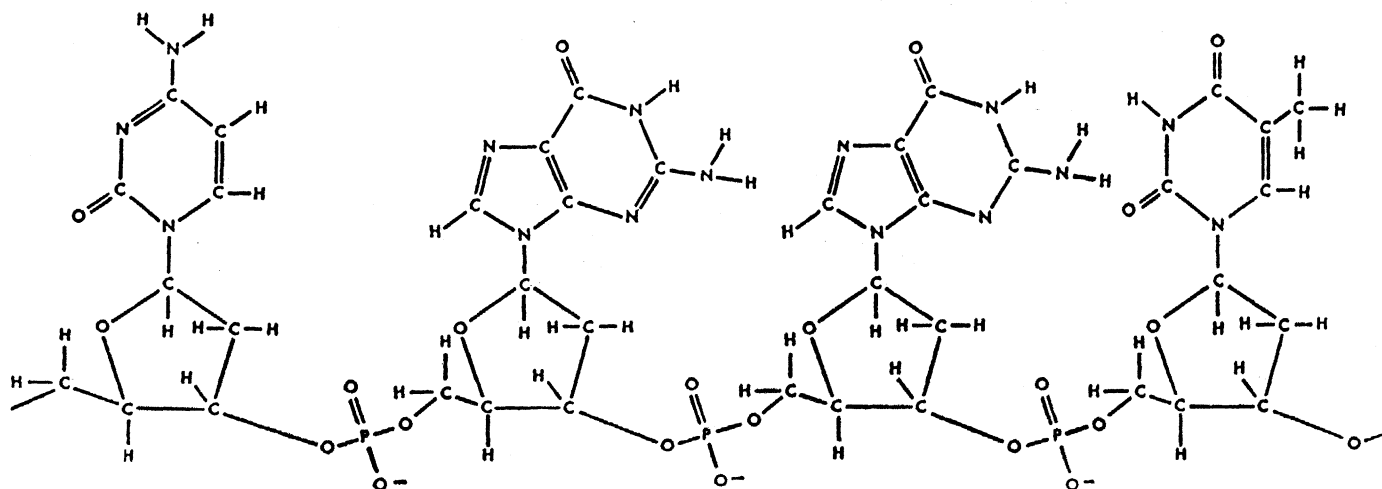
Fig. 1. Primary structure of DNA—a segment of polynucleotide sequence CGGT. [(From 13)]
