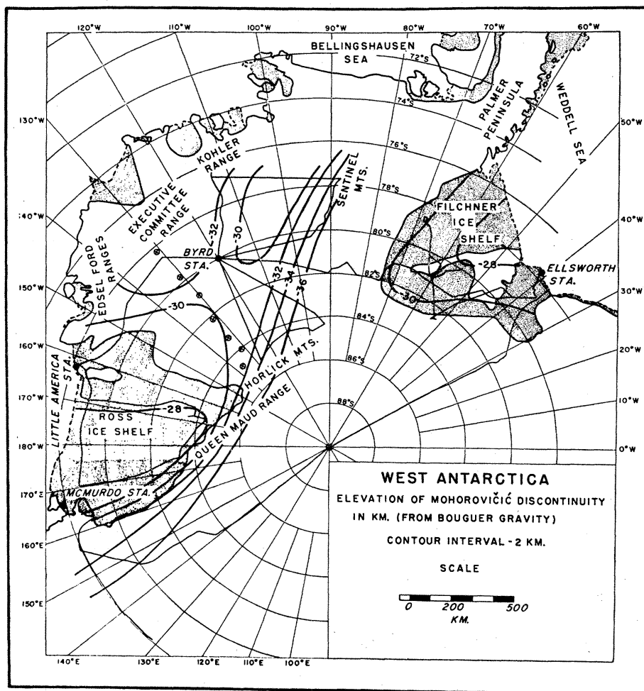
Fig. 4. Elevations of the Mohorovičić discontinuity (in kilometers).
