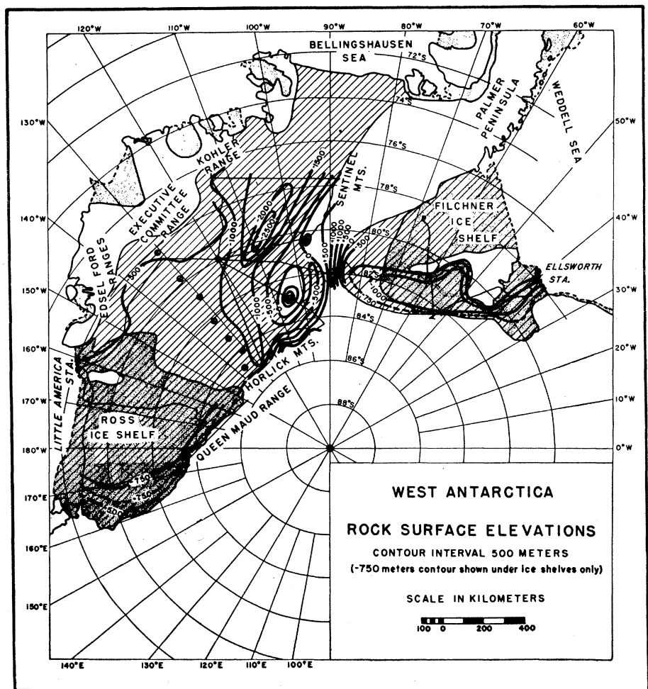
Fig. 3. Rock surface elevations in West Antarctica.
