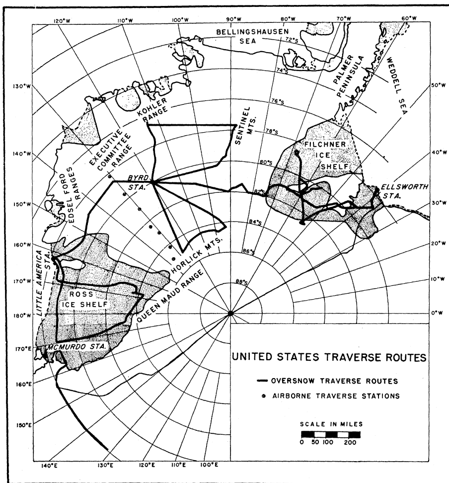
Fig. 1. Traverse routes in West Antarctica.
