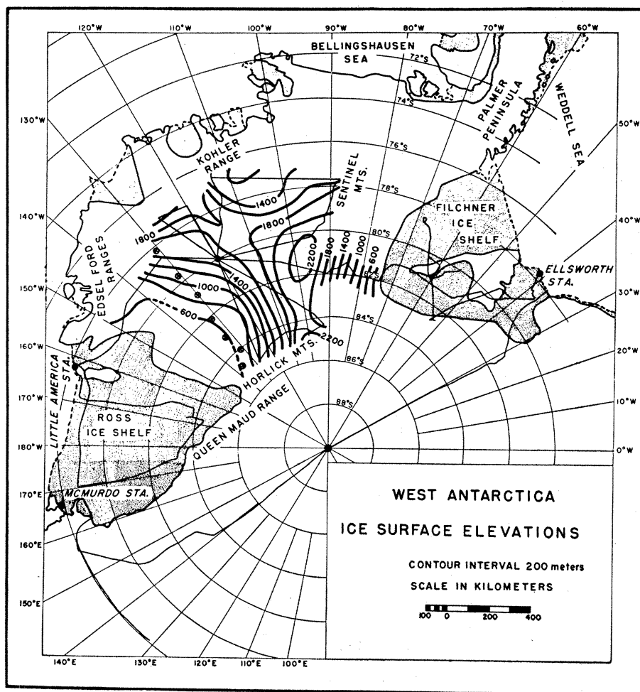
Fig. 2. Ice surface elevations in West Antarctica.
