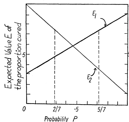
Fig. 6. Mathematical expectation of treatment.
