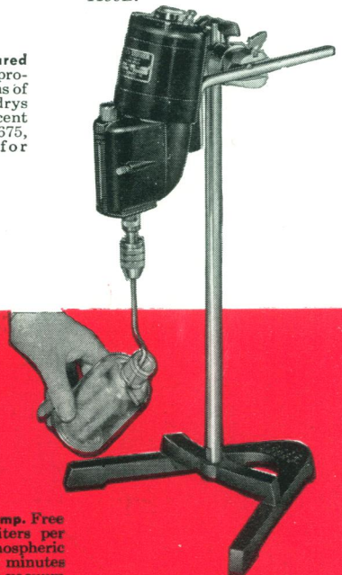
Cenco High Torque Stirrer, Improved. For light or viscous liquids. Precise control of speed from 100 to 1300 rpm. No. 18802-1, $95.00. Request Circular 1199B.
