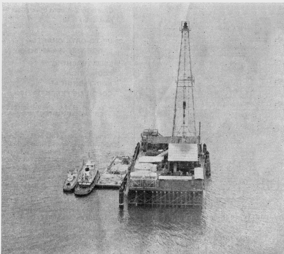
An example of off-shore drilling in the Gulf of Mexico. Shown above is Magnolia Petroleum Company's well # 1, located 5 miles off-shore from Eugene Island, off the coast of St. Mary's Parish, Louisiana. This well was recently completed as a dry hole at TD 12,874 feet.
